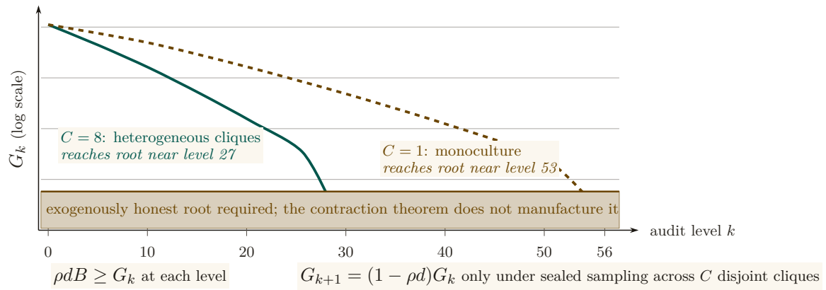
Figure 8: Recursive auditing becomes finite only when corrupt opportunity contracts. The parameterized example plots the chapter’s reported depths: heterogeneous sealed sampling across C = 8 cliques reaches the honest-root boundary near level 27, while a monoculture ( C = 1 ) requires roughly 53 levels. More boxes or more height would not prove this result; the governing conditions are local deterrence \rho dB \geq G_k and contraction G_{k+1} = (1 - \rho d)G_k . The amber floor is deliberately separate: the imported theorem bounds the tower but does not supply its exogenously honest root or the telemetry that estimates d .
