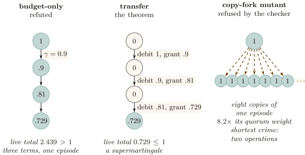
Figure 3: Three lineages of one witnessed episode of weight 1, derived at \gamma = 0.9 . Under the budget-only phrasing every derivation stays live and the closure sums to 0.9 + 0.81 + 0.729 = 2.439 > 1 : reputation minted from nothing, which is why that phrasing was refuted before proving. Under transfer each derivation grants the child \gamma w_p and debits the source w_p , so only the leaf is live and the total never exceeds what was witnessed. The copy-full mutant, which forks the undebited record, turns one episode into 8.2\times its quorum weight in two operations, and the checker refuses it. [verified for the chain by hand; internal, a6_no_mint.py , seed 20260816]
