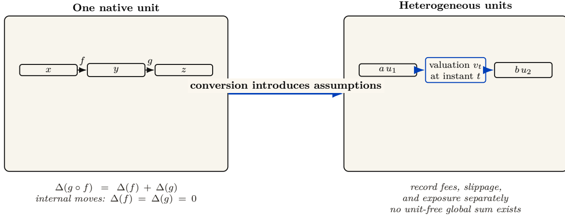
Figure 5: Conservation composes exactly within one unit of account but not across currencies without further assumptions. In one native unit, the supply delta of a composed trace is the sum of its step deltas, so zero-delta internal operations remain conservative. A cross-currency transfer is different: it requires a named valuation function and instant, plus explicit fee, slippage, and exposure accounts. Category-theoretic language does not remove those accounting assumptions.
