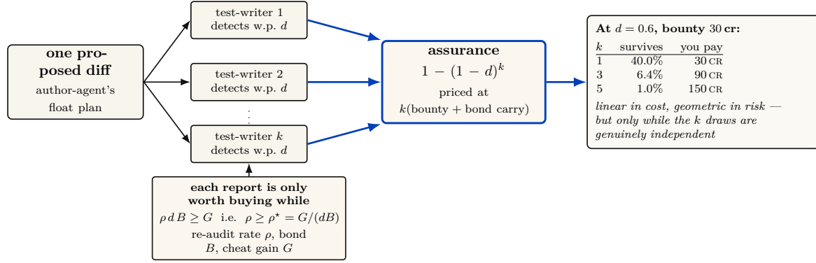
Figure 15: Assurance is bought in units of k , and the price of a unit is one bounty plus one bond carry. The mechanism is geometric on the risk side and linear on the cost side — three independent reviewers at d = 0.6 take a planted flaw’s survival odds from 40% to 6.4% for three bounties — which is why an operator can quote an assurance level as a line item at all. Two conditions carry the whole figure. The gate underneath sets what a report is worth: a test-writer is deterred from inventing or suppressing flaws only while its expected forfeiture \rho dB covers the gain G from misreporting, i.e. only while the platform commits to re-auditing at \rho \geq \rho^* = G/(dB) . And the word independent in the hypothesis is the real cost centre: correlated test-writers — same model family, shared blind spot, or visible submissions — collapse k draws toward one, so the priced assurance overstates the delivered assurance. Buying assurance means buying diversity, not headcount.
