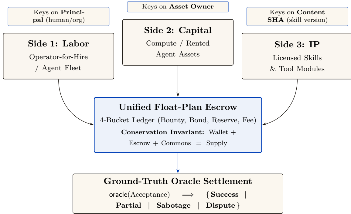
Figure 2: Labor, capital, and IP are three distinct incentive constraints — not three UI tabs — that settle on one escrow but key reputation on three different identity objects. Labor, capital (rented agents), and IP (licensed skills) all settle on a single float-plan escrow, so conservation holds globally without a second ledger. This is the categorical heart of the design: the three sides are isomorphic at the conservation object (the escrow) and non-isomorphic at the identity object (each side keys reputation on a different entity, the dashed band). Calling it “one structure, three decorations” without that qualifier is a decorative-analogy failure. The rider is mandatory: the market is three-sided by design and two-sided in shipped reality, because sides 2 and 3 presuppose a non-forgable, durable identity (§6). The economics per side: labor’s margin is bounty — slashed sub-bonds — fee; capital’s renter holds the runtime jail while the owner bears reputation; IP is metered with clawback, paid only on green settlement. The escrow and its conservation invariant are implemented and property-tested.
