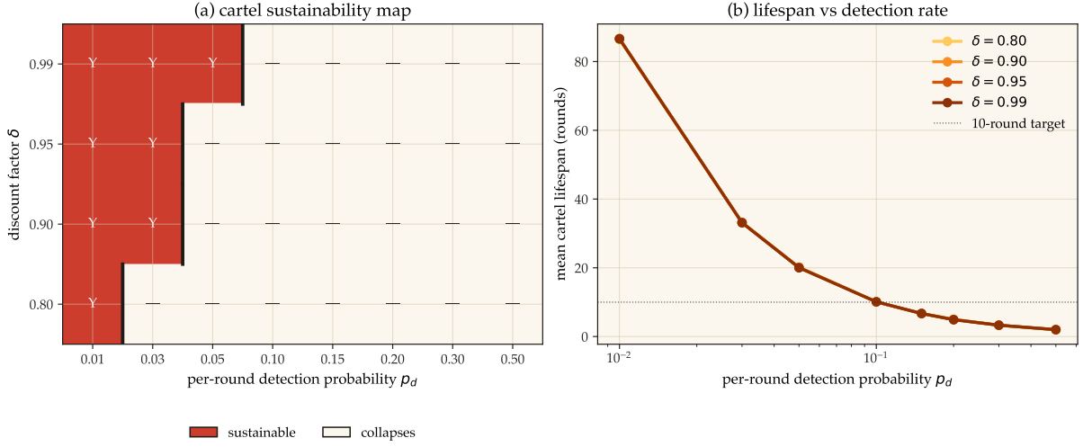
Figure 8: A6 — Repeated-game cartel folk-theorem. Left: sustainability map over the (p_d, \delta) grid; red cells are configurations where the grim-trigger cartel beats one-shot defection in expected PV (sustainable), white cells are where it does not (collapses). The thick black vertical bars mark the per-row threshold p_d^* . Right: mean cartel lifespan (rounds until first detection) vs. p_d , one line per discount factor \delta . At the realistic \delta = 0.95 , p_d^* \approx 0.10 : protocols must achieve \geq 10\% per-round detection to break repeated-game cartels.
