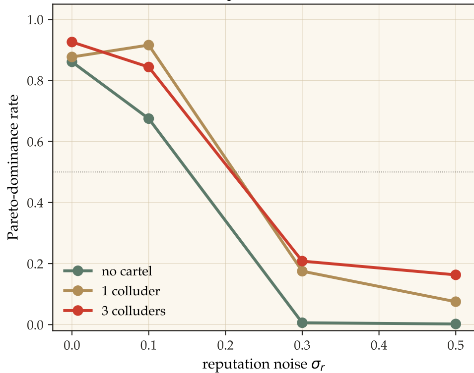
(a) dominance vs reputation noise ( n=5 insurers)
