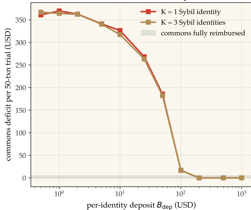
A5 — Sybil attack: deposit-only deterrence has a coverage-bounded ceiling (a) attacker net vs deposit (cap-bounded) (b) commons deficit vs deposit
