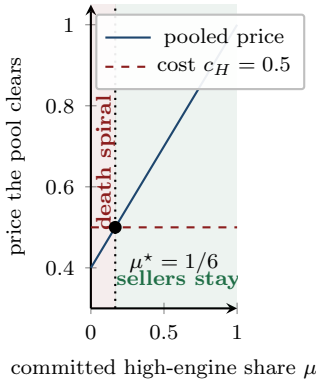
Figure 3: Regime diagram for Theorem 2 at the worked instance. Left: unattested, the pooled price clears c_H only right of \mu^* = 1/6 ; left of it the spiral rests at \theta_L . Right: the swap gain is a price-independent \Delta c without attestation and \Delta c - \Delta\theta with it — negative exactly when the strong engine is efficient, so the market’s incentive and the planner’s rule coincide [verified; regenerated by paper5_figures.py ].
