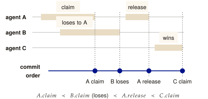
Figure 1.12: A real-time history and its extracted linearization. Operations overlap in caller time, but each receives one commit point on the single writer’s rail, and the linearization reads: A claims, B loses, A releases, C claims. The claim is conditional on one writer, no uncommitted reads, and replies after commit. [internal]
