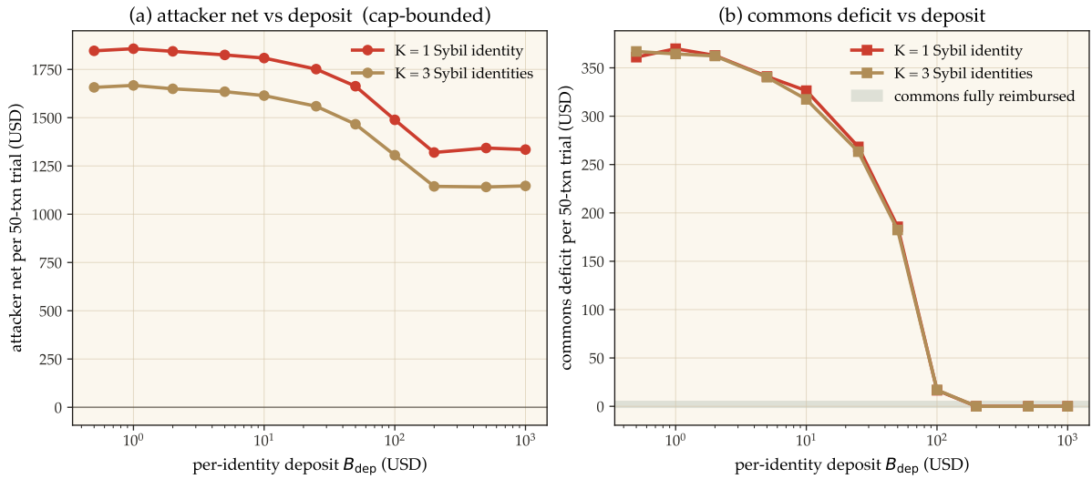
Figure 6: A5 — Sybil attack: deposit-only deterrence has a coverage-bounded ceiling. Left: attacker net profit per 50-transaction trial stays positive across the entire deposit sweep ( B_{\text{dep}} \in [0.5, 1000] USD). Right: commons deficit converges to zero around B_{\text{dep}} \approx 200 USD — the protocol is fully reimbursed, but the attacker still profits because deposit slash is capped at coverage B_T = \mu(1 + s) . Closing A5 requires a composite mechanism ( C_{\text{kyc}} + \text{reputation gating} + \text{per-class } B_{\text{dep}} ); pure deposit-based deterrence is provably insufficient.
