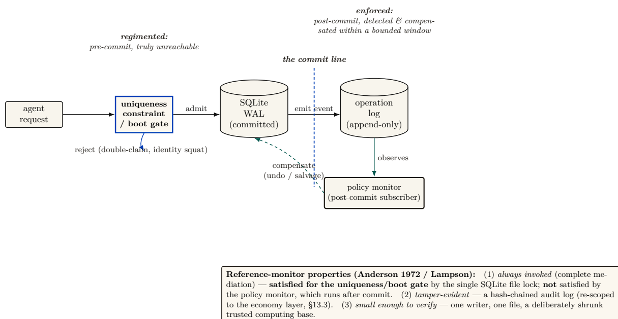
Figure 8: The kernel as a reference monitor — and the honest correction it forces. Anderson’s reference monitor must be always invoked on the request path, before the operation commits. The uniqueness constraint / boot gate (cobalt) meets this for double-claims, duplicate-identity squatting, and the serve-from-test-database guard: it rejects before the WAL write. The policy monitor (teal) does not: it is a subscriber to the operation log that fires after the event is already durable. By Schneider’s theorem [4] (§8) a monitor downstream of the commit line enforces no safety property — it can only detect and compensate . We therefore reserve “physically unreachable” for the regimented set and say “detected within a bounded window, then halted or compensated” everywhere else.
