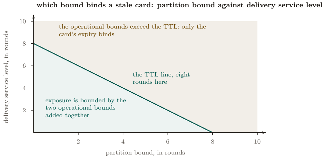
Figure 5: Which bound binds a stale card after revocation. Under a partition bound and a delivery service level, exposure is at most the two added together (Corollary 5.1); once that sum exceeds the card's time to live, the expiry binds instead and the harbor fails closed. Without a partition bound the horizontal axis is unbounded and only the expiry remains (Theorem 5.1, item 3); the line is drawn for a time to live of eight rounds.
