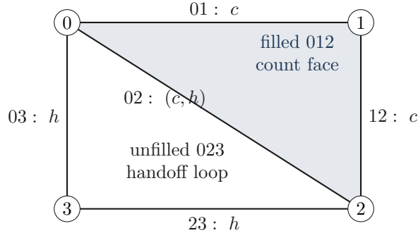
Figure 1: A heterogeneous two-complex with five physical edges and six typed edge coordinates. The 012 face compares completion counts; no face relation is declared for the 023 handoff cycle.
