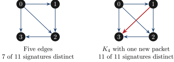
Figure 2: One independently acquired cross-edge resolves the four signed single-edge signature collisions in the finite fixture. The new packet is an additional observation, not a repair action.
