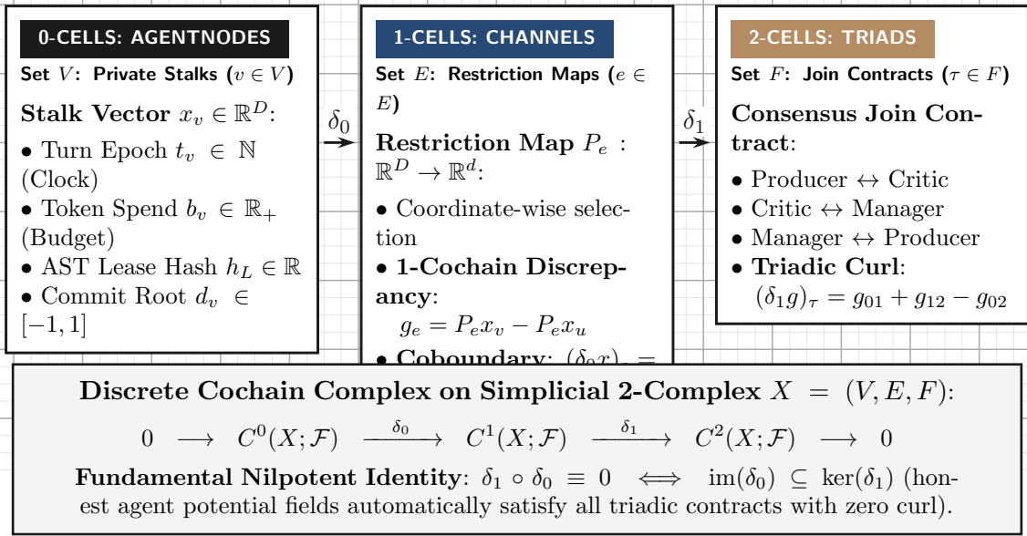
Figure 3: The Rosetta Stone conforming to Swiss Modern Systems Graphics: exact algebraic translation from multi-agent swarm primitives into cellular sheaves and simplicial complexes over cell complex X = (V, E, F) .
