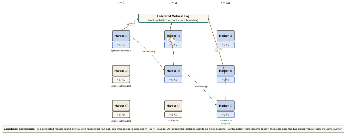
Figure 4: Federated revocation propagation across three harbors. The cuckoo filter mechanism is unchanged from Anchor §2.4 of the accompanying chapter, but two new pieces are bolted on: (a) per-epoch roots R_X^{(e)} published to a shared witness log so a third party can audit any harbor's local view, and (b) cross-witness signatures so the auditor pattern generalizes Certificate Transparency [9]. The illustrated \Delta -spaced hops are one execution, not a universal deadline: availability depends on overlay connectivity and delivery assumptions.
