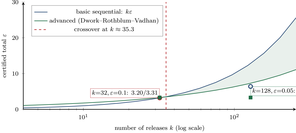
Figure 4: Regime diagram for Pillar III: which DP accounting to quote at which engagement length ( \delta' = 10^{-6} ). Below the crossover in k the sequential bound k\epsilon is exact, \delta -free, and smaller; past it, advanced composition’s \sqrt{k} scaling wins. The session’s two measured points ( k=32, \epsilon=0.1 and k=128, \epsilon=0.05 ) are marked [verified; regenerated by a3_epsilon_ledger.py ].
