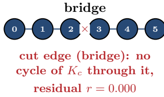
Figure 2: Regime diagram for the mechanism, in one legend with Figure 1 (harborblue solid compared, seagreen dashed relayed, gray dotted severed; the shipred \times marks the lied-on link, independently of its tier). (a) A single-edge fault on a relayed link in a visible cycle gives r = 1.225 for s = 3 . (b) The same fault on a relayed bridge gives r = 0 . (c) A severed edge has no row in K_c and cannot affect this residual. The relayed endpoint claims in (a) and (b) also permit direct sender-claim comparison when authenticated and snapshot-aligned. The figure states a one-edge residual criterion, not a unique detection advantage or a criterion for every split view [internal, sheaf_harness_v2.py].
