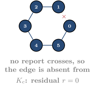
Figure 2: Regime diagram for the mechanism, in one legend with Figure 1 (harborblue solid compared, seagreen dashed relayed, gray dotted severed; the shipred \times marks the lied-on link, independently of its tier). (a) A single-edge fault on a relayed link in a visible cycle gives r = 1.225 for s = 3 . (b) The same fault on a relayed bridge gives r = 0 . (c) A severed edge has no row in K_c and cannot affect this residual. The relayed endpoint claims in (a) and (b) also permit direct sender-claim comparison when authenticated and snapshot-aligned. The figure states a one-edge residual criterion, not a unique detection advantage or a criterion for every split view [internal, sheaf_harness_v2.py].
