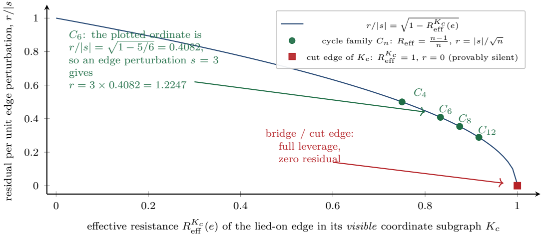
Figure 3: One-edge residual sensitivity is set by the visible topology and chosen Euclidean feature metric. The closed form plots residual per unit edge perturbation , r/|s| = \sqrt{1 - R_{\text{eff}}^{K_c}(e)} , against the effective resistance of the lied-on edge in its visible coordinate subgraph K_c — compared-plus-relayed links only, so severing a link on the edge’s cycle moves the point right, toward silence. The cycle family C_n sits at R_{\text{eff}}^{K_c} = \frac{n-1}{n} ; the marked C_6 point is the plotted ordinate 0.4082, which an absolute lie of s = 3 scales to the harness’s r = 1.2247 . The cut-edge corner R_{\text{eff}}^{K_c} = 1 is provable silence [verified; closed form exact on C_4 – C_{12} and 200 random graphs, sheaf_consistency_radius.py ].
