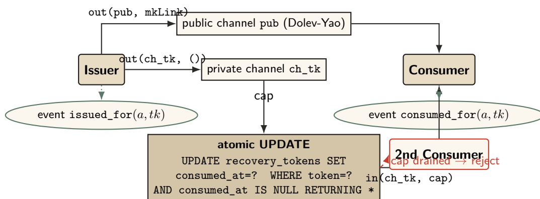
Figure 5: Magic-link single-use atomicity. The SQL UPDATE ...WHERE consumed_at IS NULL RETURNING is the runtime analogue of the ProVerif private-channel cap: SQLite serializes concurrent writers, so the first caller drains the cap and the second consumer’s transaction returns zero rows. Verified properties: injective single-use ( \text{inj-event}(\text{consumed\_for}) \Rightarrow \text{inj-event}(\text{issued\_for}) ) and binding.
