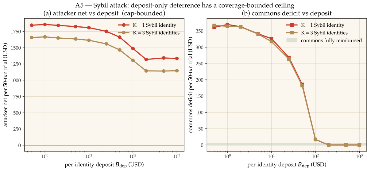
Figure 4: A5 — Sybil attack: deposit-only deterrence has a coverage-bounded ceiling. Left: attacker net profit per 50-transaction trial stays positive across the entire deposit sweep ( B_{\text{dep}} \in [0.5, 1000] USD). Right: commons deficit converges to zero around B_{\text{dep}} \approx 200 USD — the protocol is fully reimbursed, but the attacker still profits because deposit slash is capped at coverage B_T = \mu(1 + s) . Closing A5 requires a composite mechanism ( C_{\text{kyc}} + \text{reputation gating} + \text{per-class } B_{\text{dep}} ); pure deposit-based deterrence is provably insufficient.
