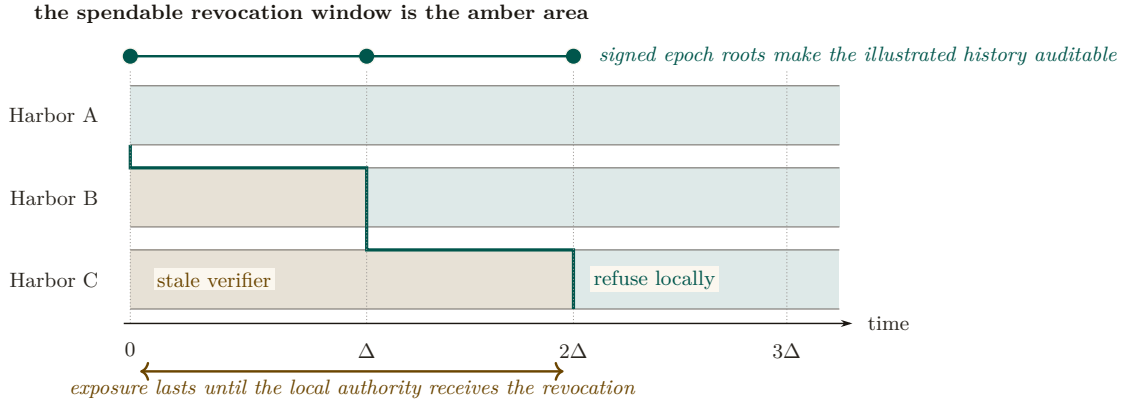
Figure 6: Revocation propagation is a moving staleness frontier. Alice refuses immediately; B remains stale until \Delta and C until 2\Delta in this illustrated execution. The amber area is precisely where a revoked capability can still be admitted by the named local authority. The teal staircase marks synchronization, not a global clock. Expected \Theta(\log m) dissemination requires connected reliable rounds; a partition can extend the amber area without bound and therefore destroys any finite deadline.
