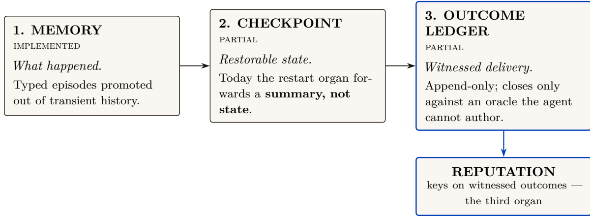
Figure III.4: The three continuity organs, honestly labelled. Memory ( implemented ) records what happened — typed episodes scored by \text{recency} \times \text{importance} \times \text{relevance} , after Generative Agents (Park 2023); checkpoint (PARTIAL) is meant to restore execution state but today passes only notes (checkpoint-of-record, not -of-execution; “with teeth” is proposed ); the witnessed-outcome ledger (PARTIAL) has durable commitments and oracle-bound closure, but not neutral graded outcome events or reputation binding. See §III.5 for the full continuity contract. It is the transitive Parfitian chain — and the organ reputation keys on. The series’ canonical seam sentence is exactly this picture in prose.
