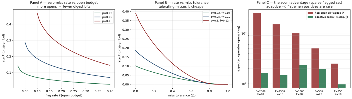
Figure 1: A: zero-miss digest rate falls as the open budget f grows. B: rate falls as miss tolerance \delta grows, exactly to 0 once f < 1 - \delta/p no longer binds (an earlier render evaluated the pinned closed form past that line and showed a spurious uptick — a domain-of-validity error, not a feature of the true frontier). C: the zoom advantage on a log scale — adaptive inspection opens far fewer items than flat when load-bearing items are sparse in the flagged set, which is exactly the regime a miss-averse (safe) digest operates in.
