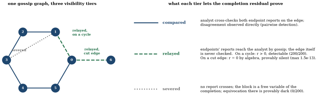
The three-tier observability contract [internal, sheaf_harness_v2.py ]
