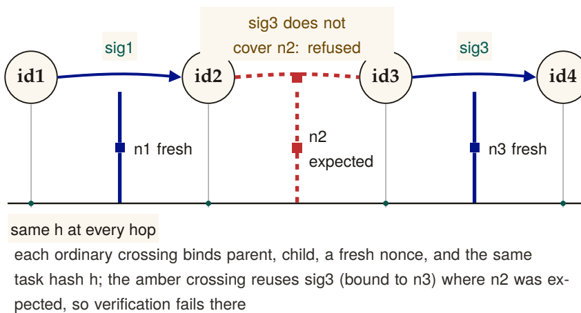
Figure 2.3: The delegation chain as a signed provenance braid across four identities \text{id1} – \text{id4} . Ordinary hops 1 and 3 bind parent, child, a fresh nonce ( n1 , n3 ), and the shared task hash h below. Hop 2 shows a splice attack: an attacker moves the legitimate signature \text{sig3} (computed over \text{id3} , \text{id4} , and n3 ) into the \text{id2} – \text{id3} position, where the verifier expects a signature over n2 ; the check fails at exactly that crossing, so the discontinuity is visible at one adjacent-identity boundary rather than anywhere else in the chain. [internal]
