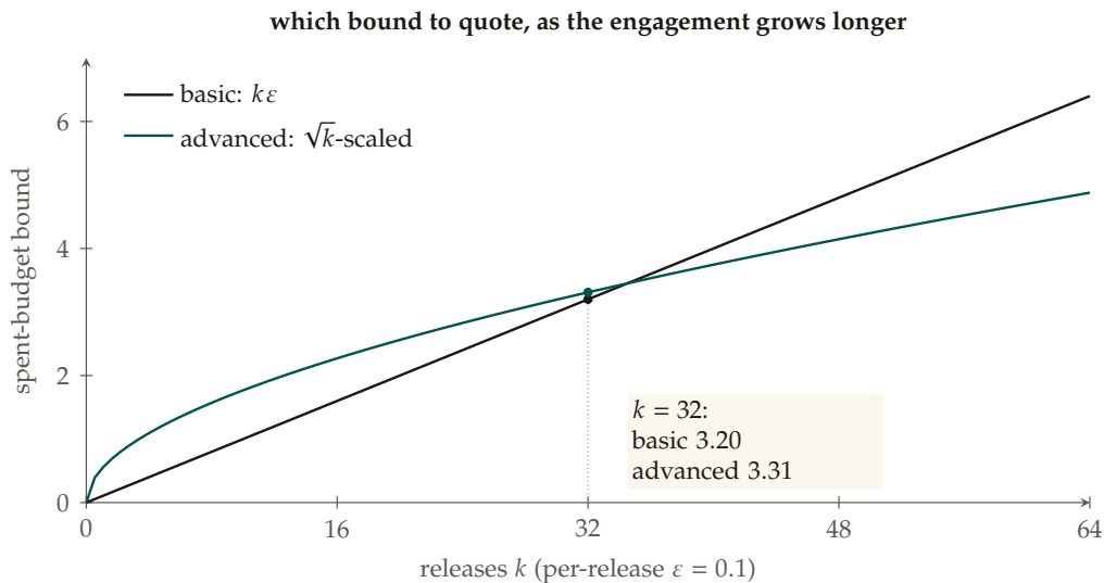
Figure 3.4: The basic and advanced \epsilon -composition bounds on cumulative spend as functions of the number of releases k , at the per-release \epsilon = 0.1 the chapter uses for this comparison. At k = 32 , the chapter’s reported comparison, basic composition (3.20) is still smaller than the advanced bound (3.31): below the crossover a contract should quote the exact, \delta -free basic bound, and only past it the square-root-scaled advanced bound – the same rule at \epsilon = 0.05 gives k = 128 : basic 6.40 versus advanced 3.30, where the advanced bound has come to pay.
