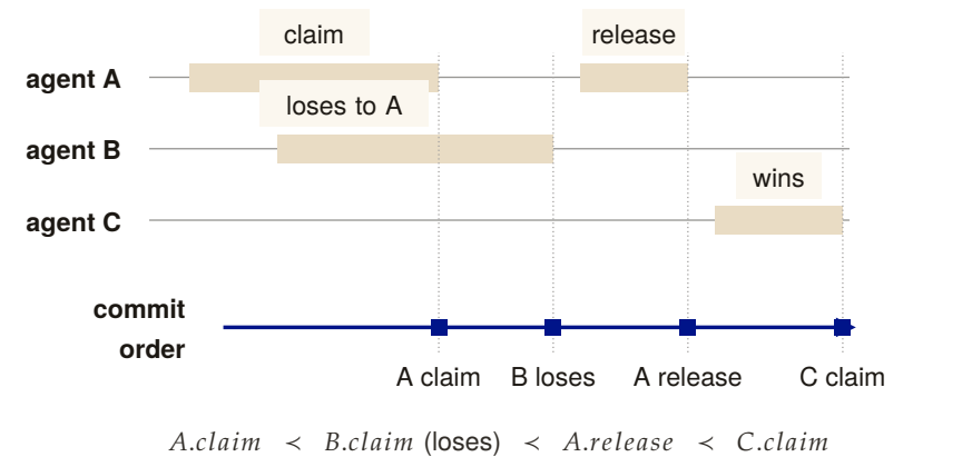
Figure 1.11: A real-time history and its extracted linearization. Operations overlap in caller time, but each receives one commit point on the single writer’s rail, and the linearization reads: A claims, B loses, A releases, C claims. The claim is conditional on one writer, no uncommitted reads, and replies after commit. [internal]
