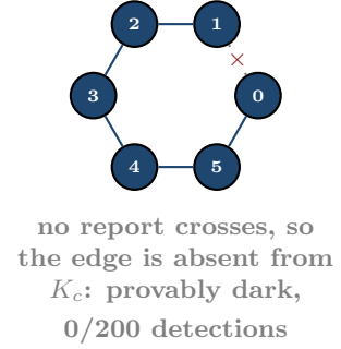
(c) C_6 , lie on a severed edge
