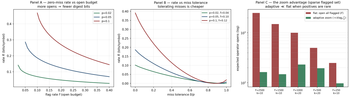
Figure 1: A: zero-miss digest rate falls as the open budget f grows. B: rate falls as miss tolerance \delta grows (the slight uptick near \delta/p \rightarrow 1 is a genuine artifact of the constraint geometry, not noise). C: the zoom advantage on a log scale — adaptive inspection opens far fewer items than flat when load-bearing items are sparse in the flagged set, which is exactly the regime a miss-averse (safe) digest operates in.
