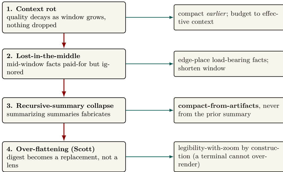
Figure 10: The context-degradation cascade (§8.3): rot makes you compact, naive compaction loses the middle, recursion fabricates, and the operator-facing digest over-flattens what’s left — the failures compound, hence “cascade.” Each rung (red) has a cure (teal), and breaking any rung stops the cascade; the load-bearing cure is compact-from-artifacts (rung 3), which a system with durable, addressable state (claims, notes, episodes) makes cheap. Cost and legibility share this surface: when compaction fails, the bill and the truth degrade together.
