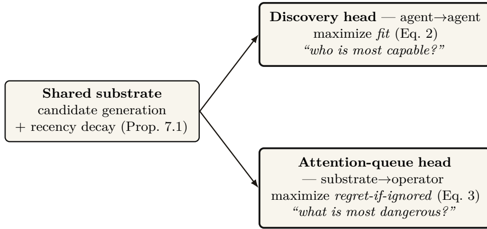
Figure 8: The split ranker (Thm. 7.1). The discovery ranker and the operator’s attention queue share candidate generation and recency-decay (Prop. 7.1) over the same signals — claims, skills, notes, episodes, presence — but apply distinct scoring heads: discovery maximizes fit (capability match, Eq. 2); the attention queue maximizes regret-if-ignored (Eq. 3). The operator wants the most dangerous item surfaced, the agent wants the most capable collaborator — incompatible loss functions, not one objective with swapped weights, so the elegant “one ranker” claim is false-as-stated and demoted to “shared substrate, distinct heads.”
