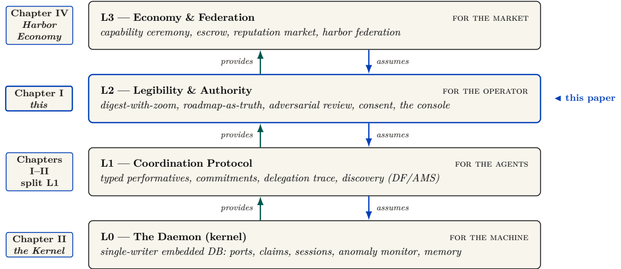
Figure 1: The four-layer stack. Each layer serves a different whom ; chapters may own or cross-cut more than one rung. This chapter owns L2 — the legibility & authority “wedge” — plus the L1 directory substrate (the existence layer that a message must address). Each layer assumes the one below it and provides to the one above: this paper assumes the single-writer kernel (the companion protocol chapter, The Single-Writer Kernel ) and provides the legible, checkpointed, outcome-bearing identity that the reputation bridge ( From Spawn to Person ) and the market ( The Harbor Economy ) consume. Chapters V–VII cross-cut the ladder with protocol, incentive, and federation deep dives.
