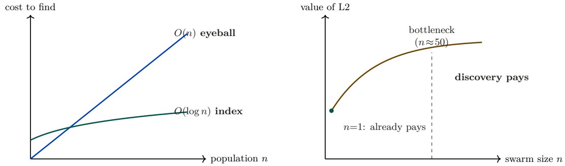
Figure 7: Read-poverty (§6): state piles up faster than it can be read. Left: the cost of finding the right agent/work grows linearly under eyeball search but stays near-flat under an indexed directory — the same trade every database made at the table-scan wall. Right: the value curve of the legibility wedge across swarm size. It is valuable already at n=1 (briefing, attestation, footgun guard, honest completion) and grows into the read-poverty regime; discovery ranking earns its keep around the n \approx 50 bottleneck. The wedge must work at n=1 and grow gracefully.
