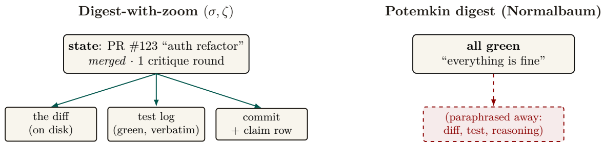
Figure 3: The one law (Def. 3.1) made concrete. Left: a legible digest line summarizes only administrative state and exposes a total zoom \zeta — every claim reaches an operator-verifiable artifact (diff, test log, commit) — mêtis preserved, the lie catchable. Right: the Potemkin digest paraphrases the work away; \zeta is partial, the summary became a replacement rather than a lens , and the tile asserts a reality with no zoom path back to ground truth. This is Scott’s Normalbaum : gloriously legible to the yield table, fatal because it erased what it could not see.
