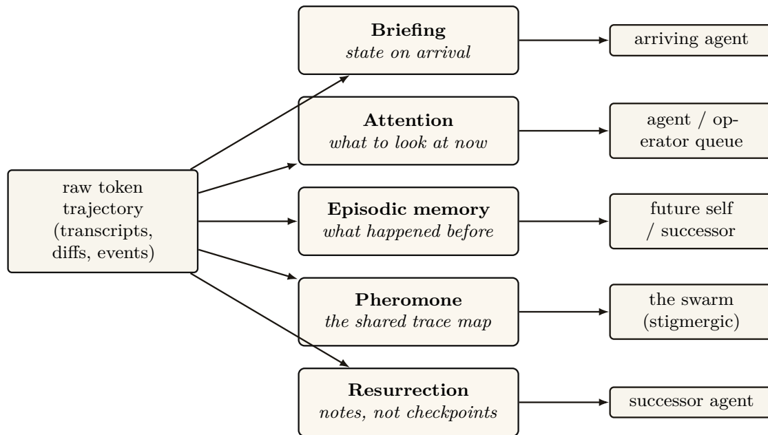
Figure 9: Five read-surfaces, each a token-compaction of the raw trajectory produced for a specific reader (§8.2): briefing is external note-taking, attention is precision compaction, episodic memory is recall-then-precision, pheromone is time-decay (forgetting), resurrection is a handoff summary. Viewed correctly, the swarm’s coordination layer is a distributed compaction engine — and because each surface is a compaction, each is governed by the same cost-and-legibility economics, the same recency-decay (Prop. 7.1), and the same one law (Def. 3.1).
