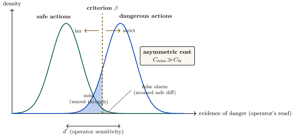
Figure 6: The operator’s forced-zoom decision as Signal Detection Theory (Def. 5.1, Eq. 1). Most actions are safe (left curve); a few are dangerous (right). The operator’s read places each action somewhere on the evidence axis; the criterion \beta decides zoom-or-wave. A lax \beta minimizes attention-seconds but maximizes misses — the danger-optimizing degenerate the naive “seconds-per-decision” objective rewards. A miss is irreversible damage; a false alarm is wasted seconds. Because C_{\text{miss}} \gg C_{\text{fa}} , the optimal criterion sits at minimal expected cost (Eq. 1), well to the left of the throughput optimum: the miss-cost term is what forces the zoom . Sensitivity d' (curve separation) is improved by better legibility; \beta is the policy knob p(r, s, v) .
