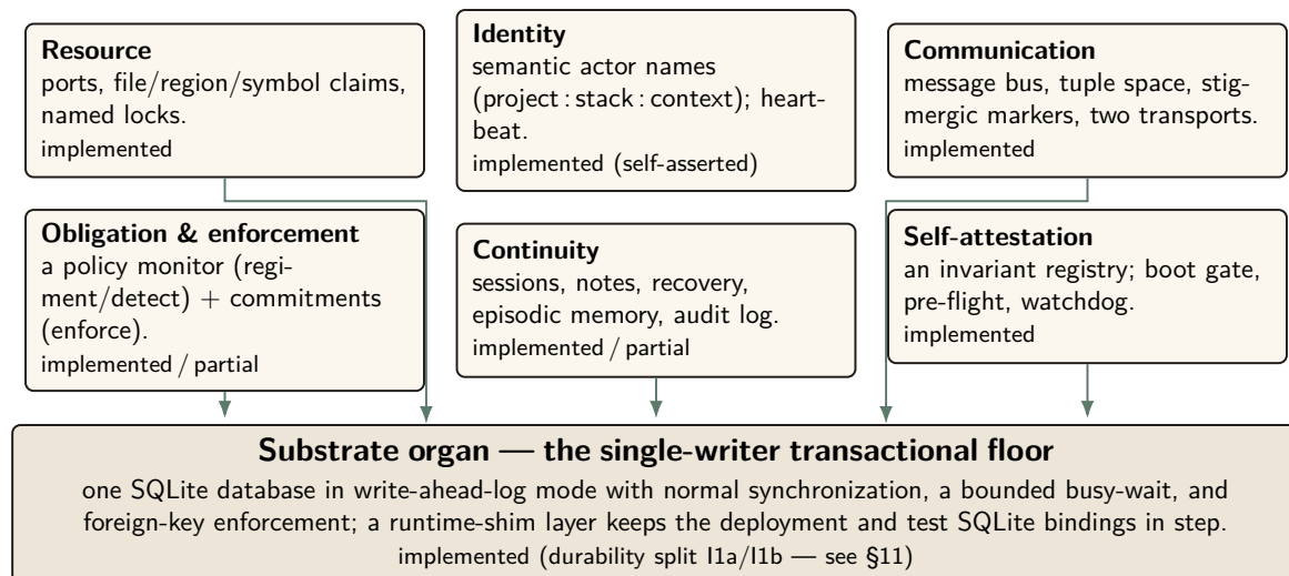
Figure 2: The kernel as seven organs , each a contract the daemon must hold for the layers above to be coherent. Six organs are, mechanically, just tables with discipline over a single shared file — the substrate organ , the single-writer transactional floor. The substrate’s storage configuration is the kernel’s durability claim; everything else is convenience built on top of it. Maturity grades (implemented · partial · specified · proposed) are per organ; note that the identity organ is implemented but self-asserted , the gap a cross-machine economy must eventually close with cryptographic identity.
