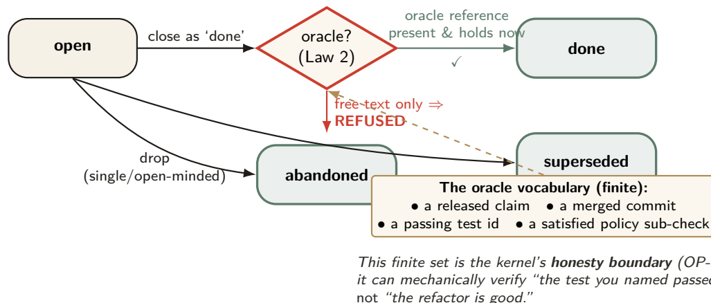
Figure 9: The commitment lifecycle with its oracle-bound closure gate. A commitment is a durable, violable promise (Cohen & Levesque’s persistent goal): it may end done , abandoned , or superseded . The load-bearing gate is Law 2: a transition to done is refused unless the agent supplies a reference drawn from a finite oracle vocabulary — a released claim, a merged commit, a passing test identifier, or a satisfied policy sub-check — that the daemon re-verifies at closure time. Free-text notes cannot close a promise. That finite vocabulary is precisely the kernel’s honesty boundary: it can verify “the test you named passed,” never “the work is good” (open problem OP-5). Law 1 (daemon-derived deadlines) closes the complementary Goodhart hole — the agent chooses the work, the daemon chooses when it is due.
