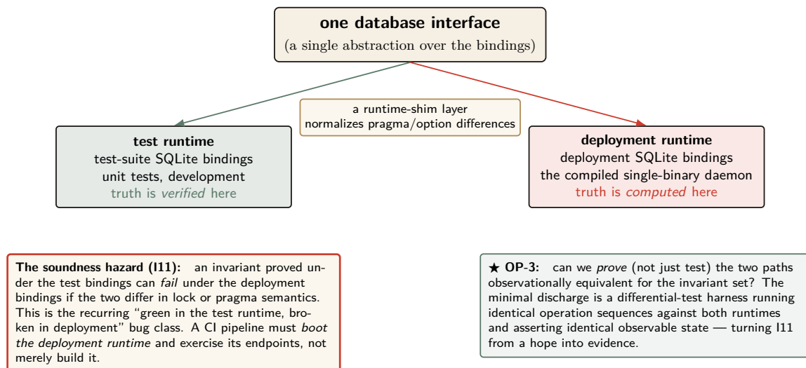
Figure 12: The dual-runtime substrate, a genuine kernel property easily mistaken for an implementation detail. One database interface is satisfied by two sets of SQLite bindings: the test-suite bindings (where invariants are verified ) and the deployment bindings in the compiled daemon (where truth is actually computed ). A shim normalizes their pragma and option interfaces, but the bridge is not a proof: an invariant green under test can fail in deployment if the bindings diverge in lock or pragma semantics — the recurring “green in the test runtime, broken in deployment” failure. Invariant I11 (runtime parity) is therefore partial , and open problem OP-3 asks for the differential-test harness that would make it a theorem.
