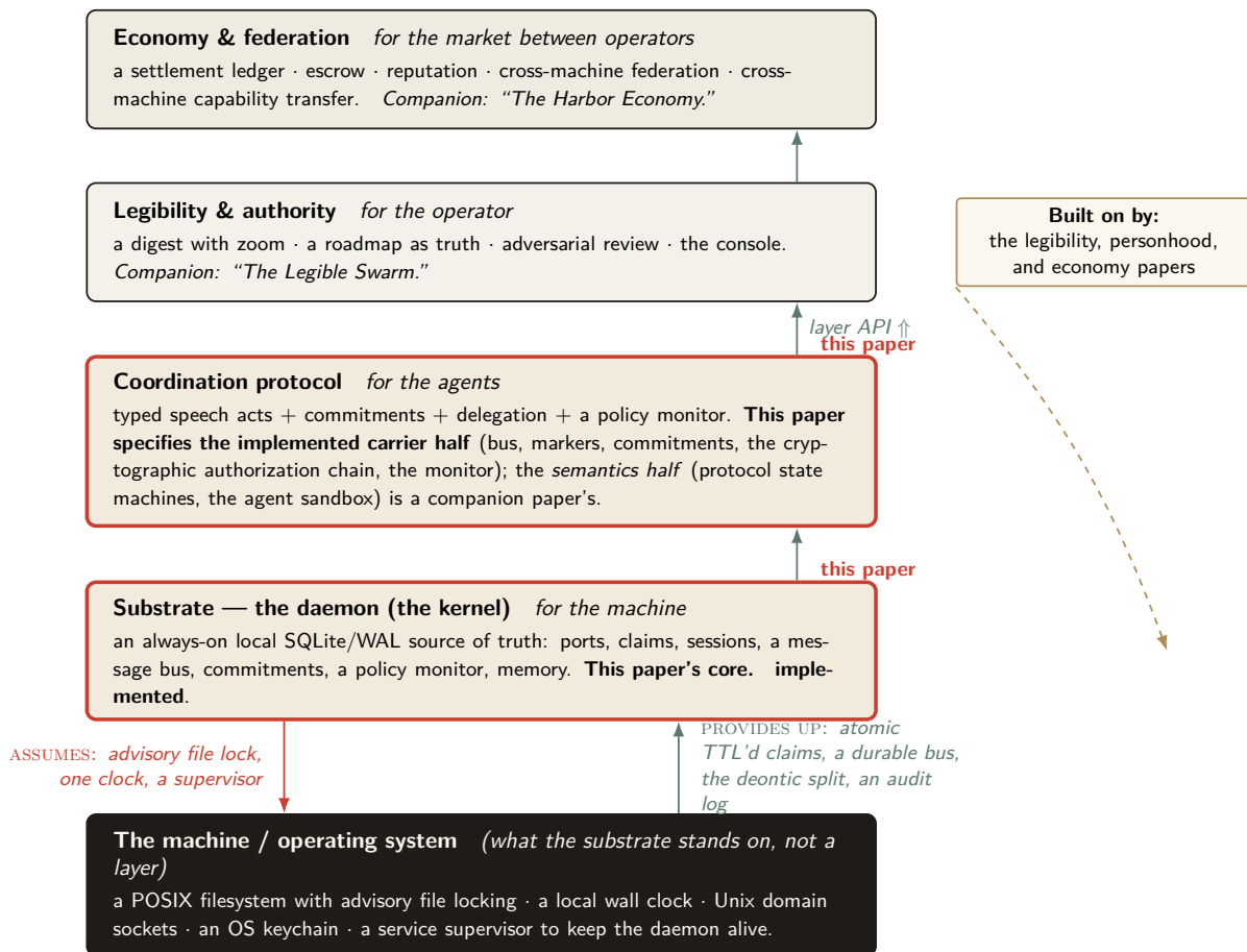
Figure 1: The four-layer coordination stack. Each layer serves a different whom (machine, agents, operator, market). This paper owns the two lowest layers: all of the substrate (the kernel) and the implemented carrier half of coordination (the message bus, stigmergic markers, commitments, the cryptographic authorization chain, the policy monitor). The coordination semantics (protocol state machines, the agent sandbox) and the whole legibility layer belong to a companion paper; cross-machine capability transfer belongs to the economy layer. Cinnabar shows what the substrate assumes from the machine; patina shows what it provides upward. Every companion paper builds on this one.
