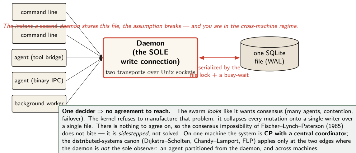
Figure 3: The single-writer serialization, the cleanest thing about the layer. Dozens of command-line invocations and agents funnel through one writer — the daemon, the sole holder of a read–write connection — and SQLite’s OS-level file lock plus a bounded busy-wait serialize all mutations. Because there is exactly one decider, there is no agreement to reach: the consensus impossibility results that dominate distributed-systems design are deliberately not substrate-layer problems. This is not a gap; it is the layer’s defining discipline. The boundary is exact: the moment a second daemon touches the same truth, you have a distributed problem — and that belongs to the cross-machine economy layer, not here.
