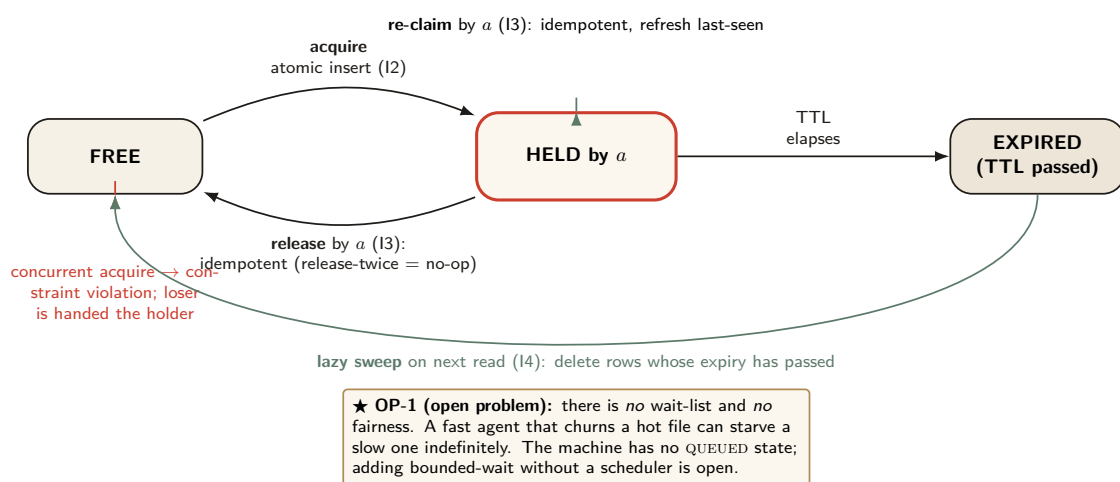
Figure 5: The claim/lock lifecycle as a finite-state machine, exhibiting the four properties on which the coordination layer builds typed ownership. Acquire is a single atomic insert against a uniqueness constraint (I2: a concurrent acquirer loses cleanly to a constraint violation and is handed the current holder). Re-claim and release are idempotent (I3): safe to retry, safe to double. Expiry is lazy-swept on the next read (I4), not on a timer. The conspicuous missing state is QUEUED: there is no fairness primitive, so a hot resource can starve a slow agent — open problem OP-1, which asks whether bounded-wait can be added without dragging a scheduler down into the kernel.
