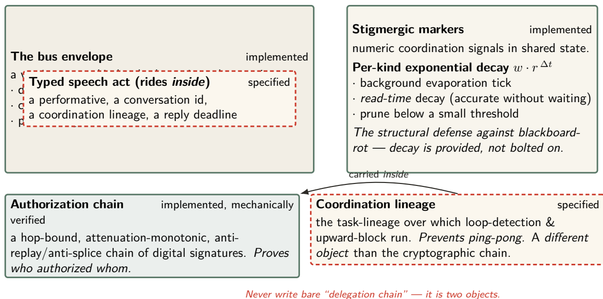
Figure 6: The communication organ. The bus envelope — durable, ordered, at-least-once, history-cursed (implemented) — is the carrier into which the typed speech act is layered; the kernel ships the envelope, the coordination layer ships the semantics that ride inside it. Stigmergic markers implement coordination with per-kind exponential decay computed both on a background tick and at read time , so the anti-blackboard-rot property is provided by the substrate rather than left to discipline. Finally, the figure fixes a dangerous naming collision: the authorization chain is the cryptographic, mechanically verified chain of signatures that proves who authorized whom ; the coordination lineage is the coordination object that prevents ping-pong — a different thing entirely, carried inside the authorization chain.
