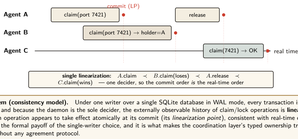
Figure 11: The consistency-model theorem — the formal property the single-writer choice buys, made explicit here. Because all mutations serialize through one writer over one WAL file, transactions are serializable ; because that writer is the sole decider, the observable history of claims and locks is linearizable : every operation has a single linearization point at its commit, and the commit order coincides with real time. The trace shows A winning a port, B losing cleanly to the holder, A releasing, and C then winning — one unambiguous order with no agreement protocol in sight. This linearizability is exactly what lets the coordination layer treat “who holds this” as ground truth.
