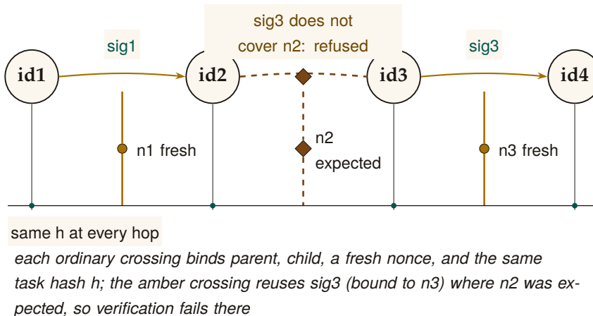
Figure 2.3: The delegation chain as a signed provenance braid across four identities id1–id4. Ordinary hops 1 and 3 bind parent, child, a fresh nonce ( n1 , n3 ), and the shared task hash h below. Hop 2 shows a splice attack: an attacker moves the legitimate signature sig3 (computed over id3, id4, and n3 ) into the id2–id3 position, where the verifier expects a signature over n2 ; the check fails at exactly that crossing, so the discontinuity is visible at one adjacent-identity boundary rather than anywhere else in the chain. [internal]
