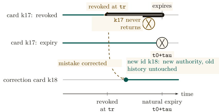
Figure 7: Acceptance is a one-way interval attached to one card ID. Card k17 stops being admissible either at explicit revocation (tick \mathbf{tr} ) or at natural expiry (tick \mathbf{t0+tau} ) and never re-enters the valid set. If revocation was a mistake, the operator issues k18 on a new lane: new authority on a new ID, with the rejected history on k17 left untouched rather than mutated. [internal]
