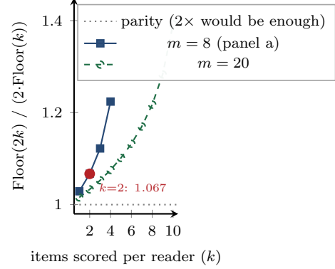
Figure 4: Split-floor comparison under one shared m -open budget. Panel (a): the excess bits for a union of disjoint critical sets over twice the single-set floor, at N=60, m=8 — 0.80 bits at k=2 and 5.72 bits at k=4 . Panel (b): the ratio over double across the plotted finite regimes. It exceeds 1 at every plotted point, reaching 1.224 at m=8, k=4 and 1.392 at m=20, k=10 [verified]. This does not require separate summary models or stores.
