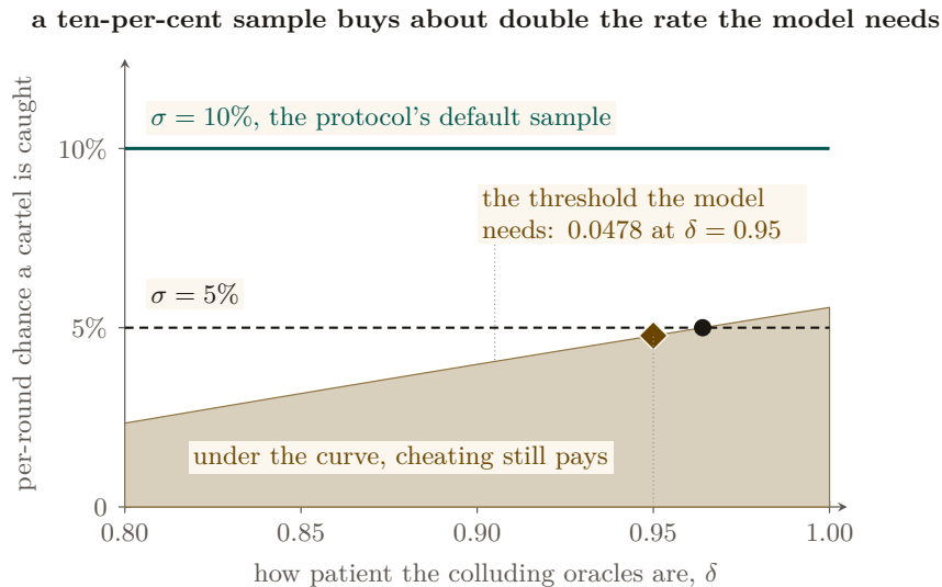
Figure 3: The default human-audit sample is roughly twice the detection rate the cartel model demands, and a halved sample is not. The amber curve is the chapter’s own fragility threshold, the per-round detection probability at which a colluding oracle pair stops preferring the cartel, drawn from (\pi_C - (1 - \delta)\pi_D)/(L + \delta\pi_D) at the supplied payoffs \pi_C = 5/3 , \pi_D = 4.95 , L = 25 ; below it collusion still pays. Because the human-audit sampling rate is the oracle layer’s detection probability, the protocol’s default \sigma = 10\% is the flat teal rule, and it clears the threshold at every patience the model admits – 0.0478 at \delta = 0.95 , and never more than 0.0557 even as \delta \rightarrow 1 . A 5% sample clears it only until \delta = 0.964 ; past that the cheaper sample silently licenses exactly the 2-of-3 oracle collusion the audit exists to price. The threshold is model-conditional: a different payoff spread, event timing, or monitoring model moves the whole curve, and the deployed detector is not claimed to attain it. [verified; figures/data/oracle-audit-threshold.csv from figures/data/make-figure-data.py, deterministic]
