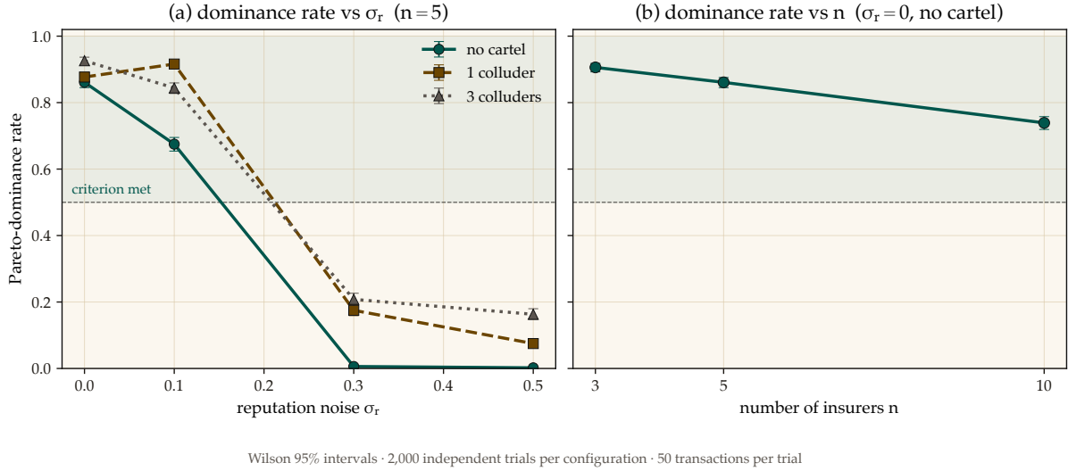
Figure 4: The competitive auction’s Pareto-dominance advantage is real but narrow: it survives moderate reputation noise and a modest cartel, then collapses once noise crosses roughly \sigma_r = 0.1 , and it shrinks as more insurers are added rather than growing. Left: fraction of trials satisfying the code’s Pareto criterion versus reputation noise \sigma_r at n = 5 , split by cartel size. Right: the same criterion versus insurer count at \sigma_r = 0 with no cartel. Error bars and seeds are recorded in the accompanying artifact; the curves are not analytical welfare bounds.
