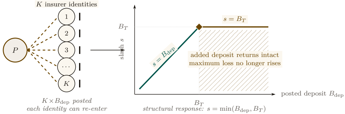
Figure VI.6: Deposit-only Sybil deterrence saturates. One principal can fund K interchangeable identities, but the loss attached to a defaulting identity rises only until its deposit reaches the transaction coverage B_T . Past that knee, s = \min(B_{\text{dep}}, B_T) = B_T : additional posted capital returns intact on no-loss transactions and cannot increase the attacker’s maximum loss. Figure VI.7 shows the corresponding simulated profit and commons-deficit sweeps.
