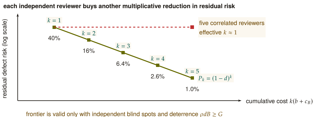
Figure 6.5: Purchased assurance is one risk-cost trajectory. Each gold point adds one independently bonded reviewer: cumulative cost rises linearly while residual defect risk falls geometrically. At d = .6 , three reviewers leave 6.4% residual risk and five leave about 1%. The dashed red counterfactual charges for five correlated reviewers but delivers roughly one reviewer’s protection. Independence and Becker deterrence \rho dB \geq G are therefore conditions of the frontier, not footnotes to headcount.
