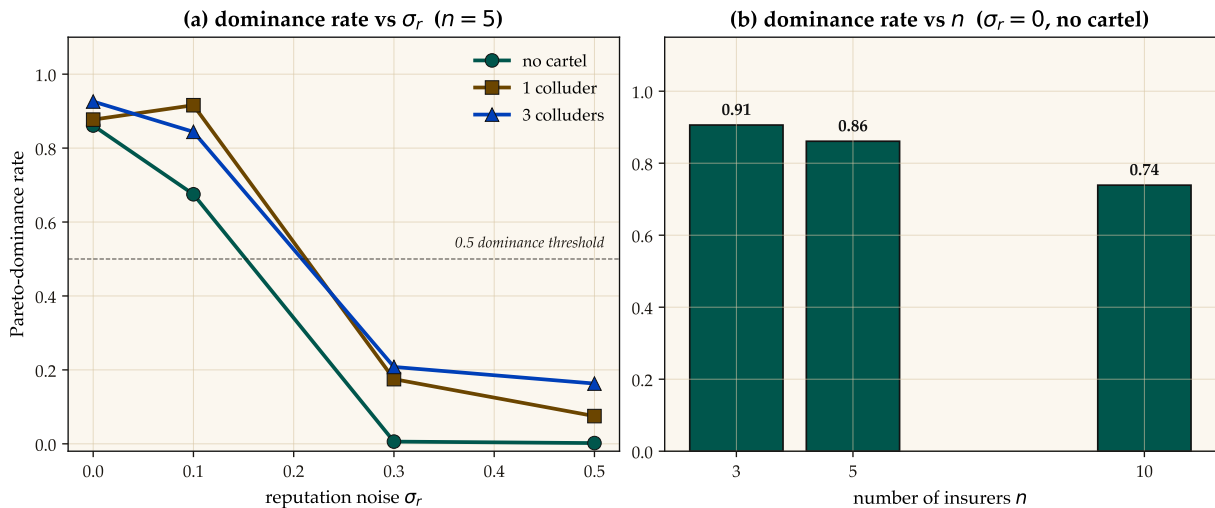
Figure VI.5: Monte Carlo comparison of competitive auction and the specified static-escrow baseline. Left: fraction of trials satisfying the code’s Pareto criterion versus reputation noise \sigma_r at n = 5 , split by cartel size. Right: the same criterion versus insurer count at \sigma_r = 0 with no cartel. Error bars and seeds are recorded in the accompanying artifact; the curves are not analytical welfare bounds.
