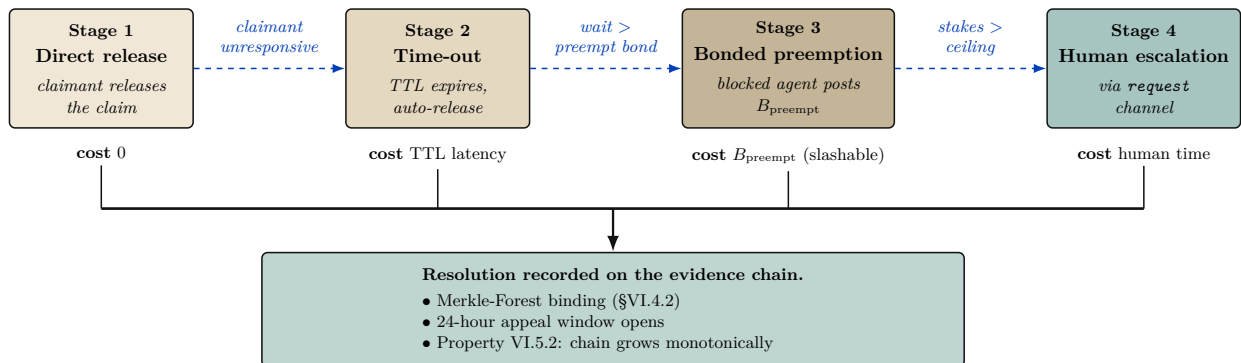
Figure VI.3: Governance and appeals: four-stage escalation path. The daemon resolves most disputes at stage 1 or 2 (zero or near-zero cost). Bonded preemption (stage 3) prices the blocked agent’s claim that the holder is wrong; if the preemption is wrong, the bond is slashed under settlement. Human escalation (stage 4) is reserved for the cases the daemon cannot mechanically decide. Every resolution is appended to the evidence chain with the same Merkle-Forest binding as any agent action, so all four stages remain auditable.
