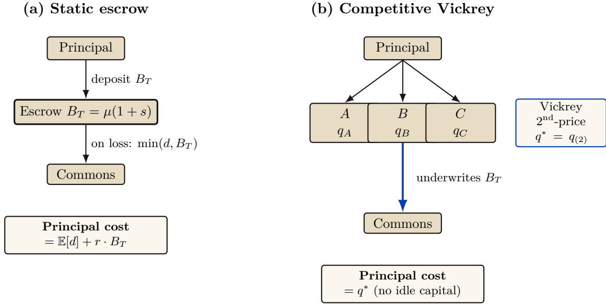
Figure VI.4: Static escrow vs. competitive Vickrey auction. Both regimes underwrite the same coverage B_T = \mu(1 + s) ; only the financing mechanism differs. In (a) the principal ties up B_T for the coverage period, paying an opportunity cost r \cdot B_T . In (b) insurers compete; the principal pays only the second-lowest bid q^* . The competitive regime Pareto-dominates the static one under the welfare assumptions of §VI.7.5.8 below.
