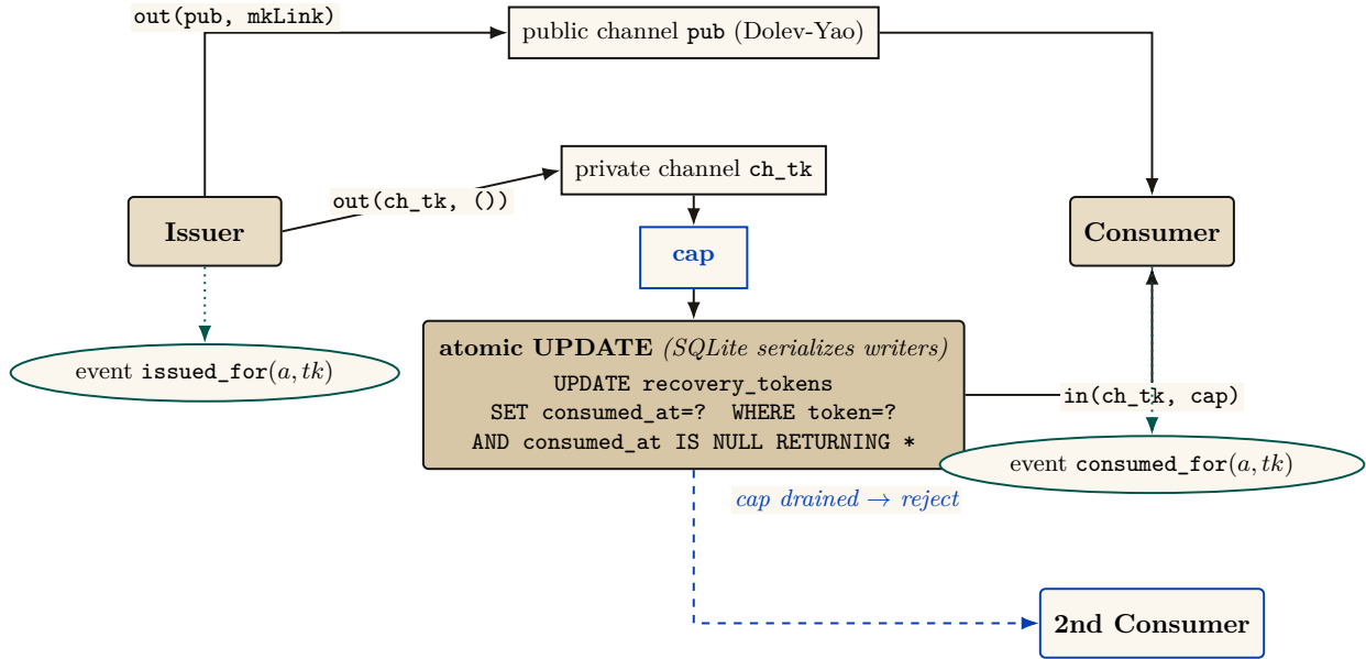
Figure VI.11: Magic-link single-use atomicity. The SQL UPDATE ...WHERE consumed_at IS NULL RETURNING is the runtime analogue of the ProVerif private-channel cap: SQLite serializes concurrent writers, so the first caller drains the cap and the second consumer's transaction returns zero rows. Verified properties: injective single-use ( \text{inj-event}(\text{consumed\_for}) \Rightarrow \text{inj-event}(\text{issued\_for}) ) and binding.
