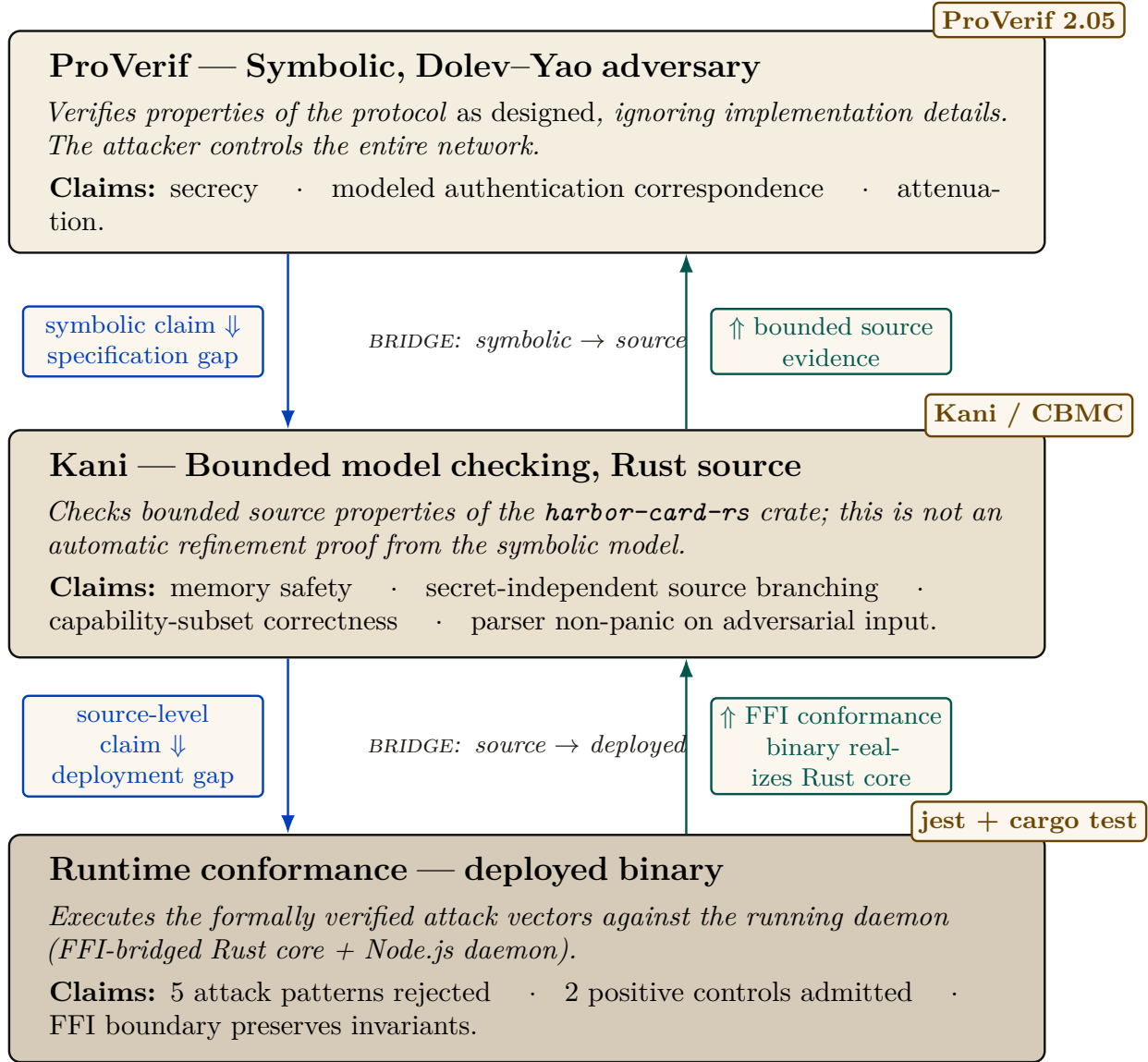
Figure V.8: The three-layer verification stack. ProVerif (top) discharges design-level obligations against a Dolev–Yao adversary. Kani (middle) checks bounded Rust source-level properties that overlap with, but do not refine the full symbolic model. Runtime conformance tests (bottom) exercise the FFI-bridged binary with selected attack vectors; they reduce rather than eliminate the deployment gap. Cobalt arrows show obligations flowing down (what each lower layer must preserve); teal arrows show evidence flowing back up. The unproved bridges remain explicit assurance-case assumptions rather than inferred theorems.
