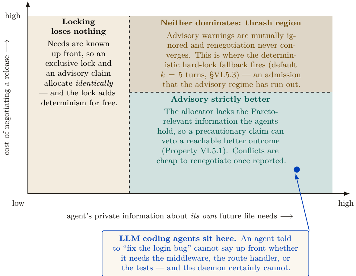
Figure VI.2: Advisory claims do not beat enforced locks everywhere — they beat them only to the right of the dashed vertical, where agents hold private information the allocator cannot have. To its left, locking costs nothing and buys determinism, so Sen’s warning does not apply and this paper’s design choice would be wrong. Above the dashed horizontal, neither regime works and the hard-lock fallback of §VI.5.3 takes over. The marked point is where LLM coding agents actually sit, which is the entire argument for the advisory default of §VI.5.2.
