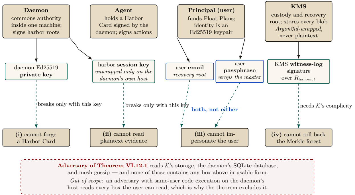
Figure VI.10: Who holds which key, and which compromise breaks which clause. Each of the theorem's four negative guarantees fails to exactly one custody compromise, and only clause (iii) requires two — email and passphrase together, which is why the recovery pair is the one place the architecture depends on a conjunction rather than a single secret. The KMS is the only party that stores everything and can decrypt nothing; the daemon is the only party that ever holds the harbor session key unwrapped, which is precisely why the theorem must exclude the same-user adversary on the daemon's host.
