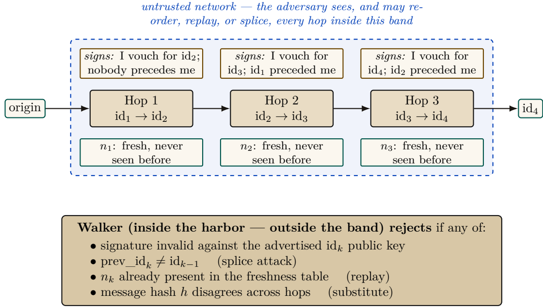
Figure V.4: Multi-hop delegation walker. Each hop k signs the binding tuple (n_k, id_{k-1}, id_{k+1}, h) under Ed25519 — written sign_{id_k}(\text{hopBind}(n_k, id_{k-1}, id_{k+1}, h)) in Algorithm 3 — where h is the message hash that must remain constant across the chain; the boxes above each hop say in words what that tuple asserts. The dashed band is the trust boundary of §V.5.1: the whole chain is adversary-visible in transit, which is precisely why each hop must bind its neighbours rather than merely follow them. The walker runs inside the harbor, verifies depth- N chains against a nonce-freshness table, and rejects splices, replays, hop-swaps, and substitution. Runtime: lib/delegation-chain.ts ; ProVerif conformance test passes 17 / 17.
