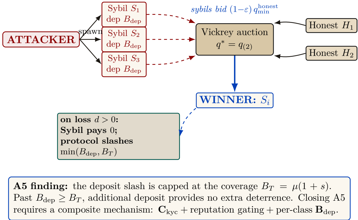
Figure VI.6: Sybil attack flow. The attacker spawns K Sybil identities, each posting deposit B_{\text{dep}} , then undercuts honest bids by \varepsilon and defaults on loss. The protocol confiscates the Sybil's deposit on default, but the slash amount is capped at the coverage B_T — so beyond B_{\text{dep}} \geq B_T additional deposit provides no extra deterrence. Empirically demonstrated in Figure VI.7.
