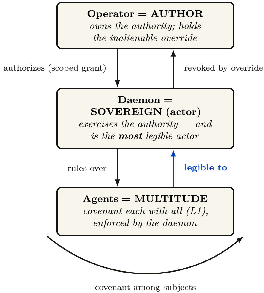
Figure I.14: Role assignment (§I.9.1) in Hobbes’ author/actor distinction ( Leviathan ch. 16). The agents are the multitude who covenant each-with-all; the daemon is the sovereign-as-actor that exercises the instituted authority — blocking, landing, escalating — but, by the legible-sovereign amendment (Prop. I.2.1), is the most legible actor, not the least — the one relation drawn in the accent color, because it is the inversion this chapter is arguing for; the operator is the author who owns the authority, issues scoped consent grants (Def. I.2.1), and holds the inalienable override (Prop. I.2.2). Naming the operator “the sovereign” would break the covenant; the author slot is the one Hobbes leaves for the one who authorizes without personally acting.
