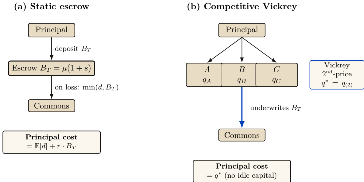
Figure IV.13: Static escrow vs. competitive Vickrey auction. Both regimes underwrite the same coverage B_T = \mu(1 + s) ; only the financing mechanism differs. In (a) the principal ties up B_T for the coverage period, paying an opportunity cost r \cdot B_T . In (b) insurers compete; the principal pays only the second-lowest bid q^* . The competitive regime Pareto-dominates the static one under the welfare assumptions of §IV.12.1 below.
