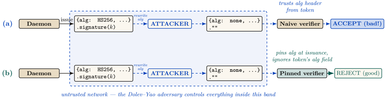
Figure V.3: Algorithm-confusion attack and the pinned-verifier defense. The dashed band is the chapter’s trust boundary: the daemon and the verifier sit outside it, and everything inside it is under the control of the Dolev-Yao adversary of §V.5.1, who may read, rewrite, or inject any token in flight. (a) A naive verifier trusts the alg field of the incoming token; an attacker inside the band rewrites alg=HS256 to alg=none , strips the signature, and the verifier accepts an unauthenticated message. (b) The pinned verifier records the issuance algorithm out-of-band — across the boundary, where the adversary cannot reach — then re-checks each token against the pinned algorithm rather than the token’s self-described one. The ProVerif model encodes both verifiers and shows the naive path produces a counter-trace witness for the rewrite, while the pinned path admits no such trace. Runtime conformance: 5 attack patterns + 2 controls, all pass.
