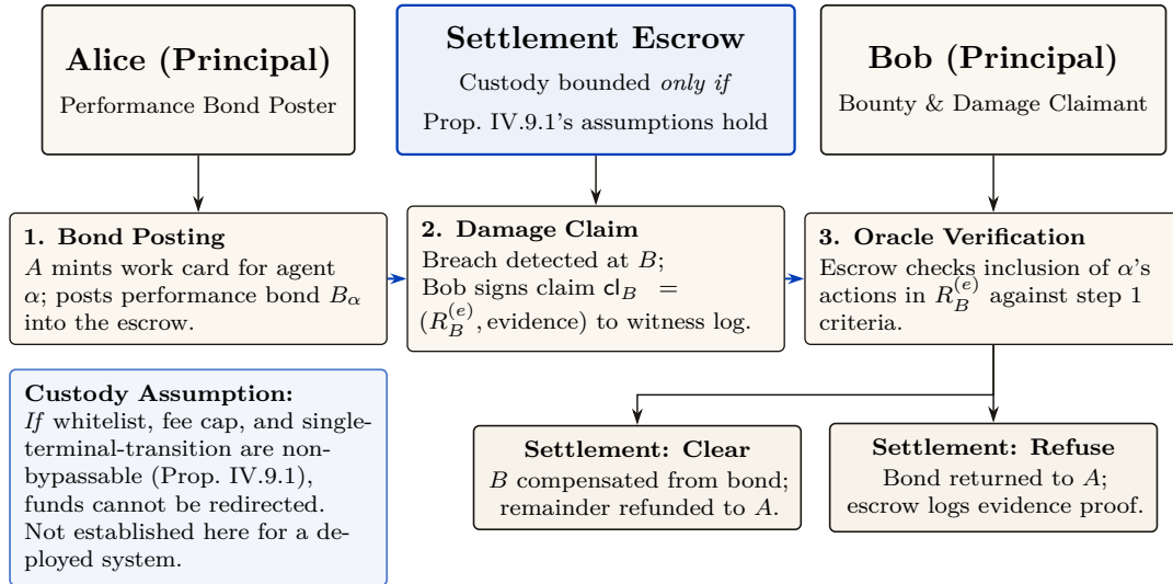
Figure IV.8: Cross-harbor settlement protocol. The custody bounds are conditional , not established: Property IV.9.1 holds only where the recipient whitelist, fee cap, and single-terminal-transition rule cannot be bypassed by the escrow operator (§IV.9.2); 2-of-3 threshold signing is one candidate way to arrange that. Under those assumptions the outcome space partitions into Clear or Refuse , bounding cross-harbor liability; without them the worst case is the full custodial balance.
