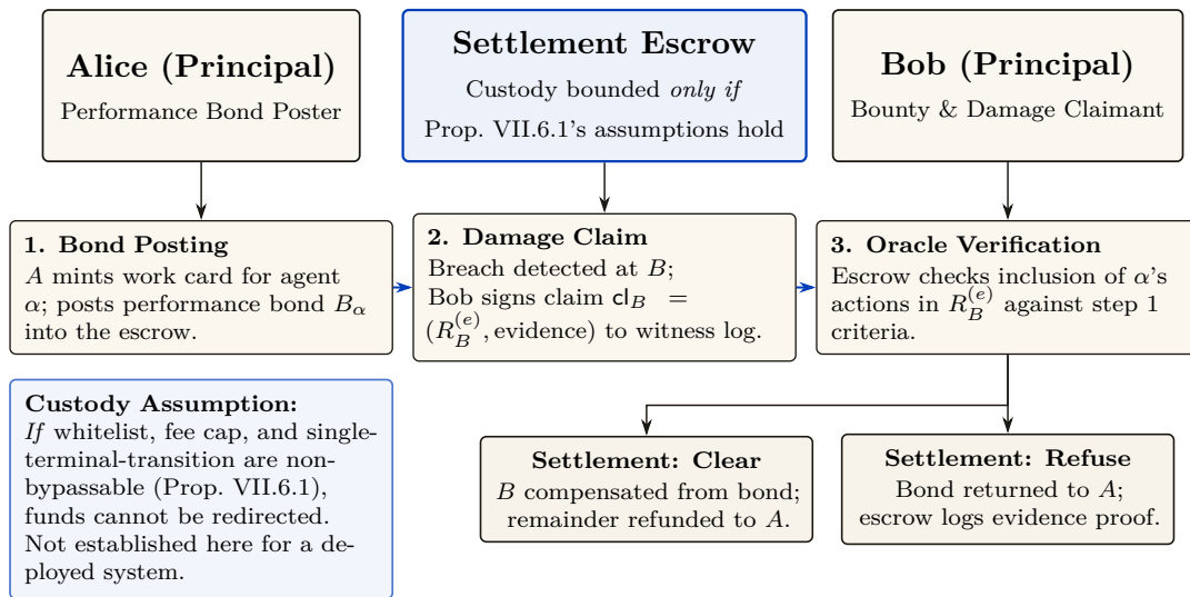
Figure VII.5: Cross-harbor settlement protocol. The custody bounds are conditional , not established: Property VII.6.1 holds only where the recipient whitelist, fee cap, and single-terminal-transition rule cannot be bypassed by the escrow operator (§VII.6.1); 2-of-3 threshold signing is one candidate way to arrange that. Under those assumptions the outcome space partitions into Clear or Refuse , bounding cross-harbor liability; without them the worst case is the full custodial balance.
