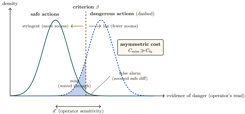
Figure 7: The operator’s forced-zoom decision as Signal Detection Theory (Def. 5.1, Eq. 3). Most actions are safe (left curve); a few are dangerous (right). Zooming triggers when evidence of danger exceeds criterion \beta . Moving \beta left is more stringent: it causes more zooms, fewer misses, and more false alarms. Moving \beta right is more lax: it minimizes attention-seconds but increases misses. Because C_{\text{miss}} \gg C_{\text{fa}} , the optimal criterion sits well to the left of the throughput optimum: the miss-cost term is what forces the zoom . Sensitivity d' (curve separation) is improved by better legibility; \beta is the policy knob p(r, s, v) .
