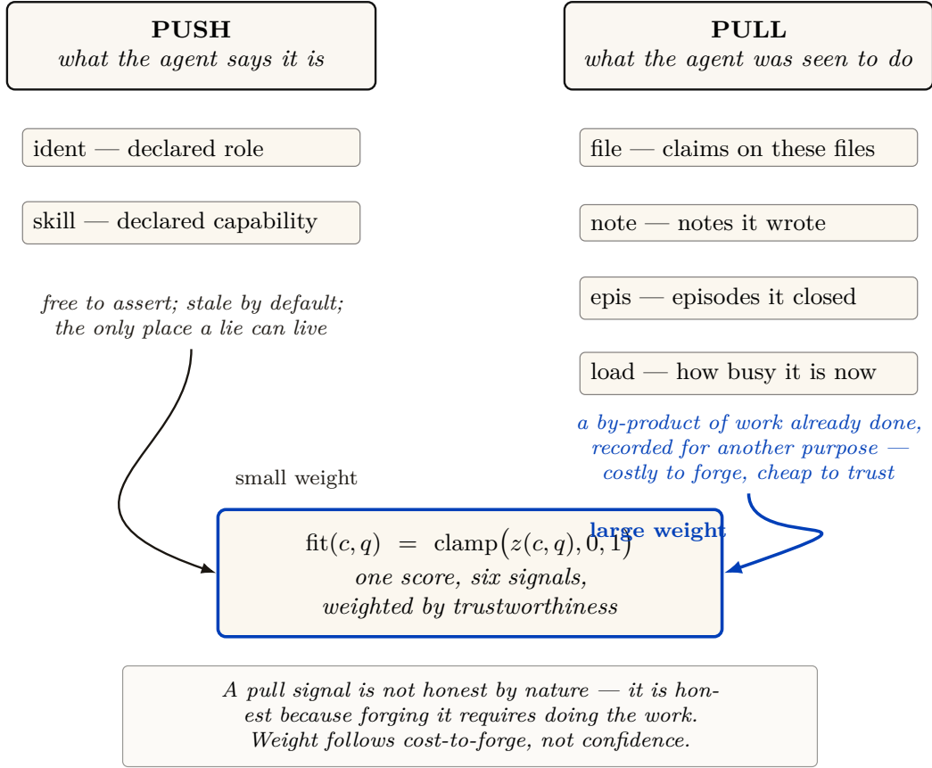
Figure 10: Push versus pull signals in the discovery ranker (Eq. 4, Table 5). Push signals are what a candidate declares about itself; pull signals are residue of work it actually did, recorded for some other purpose. The design weights pull over push not because declarations are usually false but because they are free — an agent that wants to be routed work can inflate a skill tag at no cost and cannot inflate a merged episode without merging something. This is the discovery-side instance of the same discipline digest-with-zoom (Def. 3.1) applies to summaries: trust the claim that reaches an artifact.
