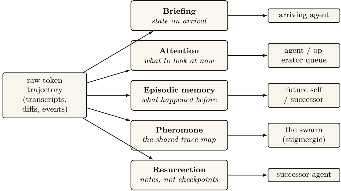
Figure 12: Five read-surfaces, each a token-compaction of the raw trajectory produced for a specific reader (§8.2): briefing is external note-taking, attention is precision compaction, episodic memory is recall-then-precision, pheromone is time-decay (forgetting), resurrection is a handoff summary. Viewed correctly, the swarm’s coordination layer is a distributed compaction engine — and because each surface is a compaction, each is governed by the same cost-and-legibility economics, the same recency-decay (Prop. 7.1), and the same one law (Def. 3.1).
