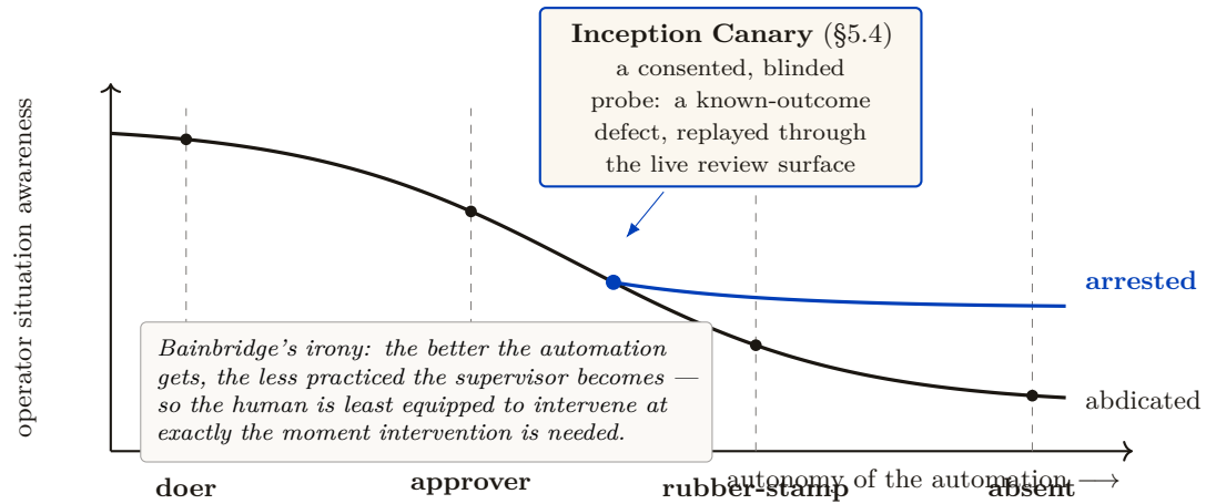
Figure 8: The abdication gradient (§5.4). As the automation takes longer plans end-to-end, the operator’s role slides through four stations — doer, approver, rubber-stamp, absent — and situation awareness slides with it. The Bainbridge–Scott convergence is that this is not operator weakness but a property of good automation : the digest erases the swarm’s métis and the operator’s alike. The design’s one active defense is the Inception Canary (Prot. 5.1), which arrests rather than reverses the slide: a consented, blinded replay of a known-outcome defect keeps the supervisor in practice without synthetic busywork. Both curves are schematic. No situation-awareness measurements exist for this system; the freeze-probe study of §5.3 is the experiment that would replace the shape with data, and until it runs this figure is an argument drawn, not a result plotted.
