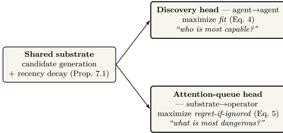
Figure 11: The split ranker (Thm. 7.1). The discovery ranker and the operator’s attention queue share candidate generation and recency-decay (Prop. 7.1) over the same signals — claims, skills, notes, episodes, presence — but apply distinct scoring heads: discovery maximizes fit (capability match, Eq. 4); the attention queue maximizes regret-if-ignored (Eq. 5). The operator wants the most dangerous item surfaced, the agent wants the most capable collaborator — incompatible loss functions, not one objective with swapped weights, so the elegant “one ranker” claim is false-as-stated and demoted to “shared substrate, distinct heads.”
