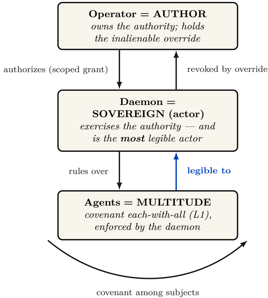
Figure 14: Role assignment (§9.1) in Hobbes’ author/actor distinction ( Leviathan ch. 16). The agents are the multitude who covenant each-with-all; the daemon is the sovereign-as-actor that exercises the instituted authority — blocking, landing, escalating — but, by the legible-sovereign amendment (Prop. 2.1), is the most legible actor, not the least — the one relation drawn in the accent color, because it is the inversion this chapter is arguing for; the operator is the author who owns the authority, issues scoped consent grants (Def. 2.1), and holds the inalienable override (Prop. 2.2). Naming the operator “the sovereign” would break the covenant; the author slot is the one Hobbes leaves for the one who authorizes without personally acting.
