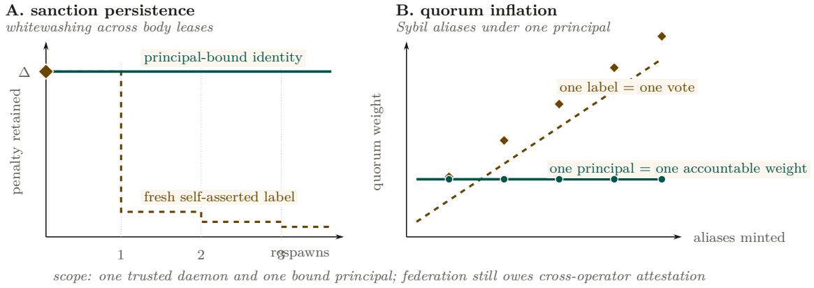
Figure 6: Non-forgable identity changes the economics of both classic attacks. In panel A, a self-asserted label drops a sanction by respawning; a principal-bound identity carries the penalty \Delta across every body lease. In panel B, free labels turn aliases into quorum weight, while principal binding keeps one accountable weight constant. The claim is deliberately local: daemon minting and principal binding close these attacks inside one trusted domain; they do not solve cross-operator attestation. Newcomer friction applies to economic ceiling, not to the ability to perform work.
