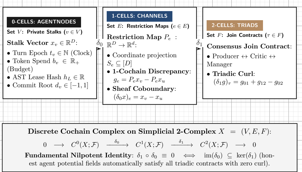
Figure 3: The Rosetta Stone: exact algebraic translation from multi-agent swarm primitives into cellular sheaves and simplicial complexes over cell complex X = (V, E, F) .
