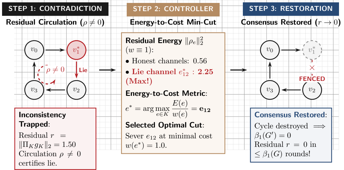
Figure 5: Theorem CR-4 active repair closed-loop cycle. (Step 1) An equivocator v_1^* injects contradiction s = 3.0 , creating non-zero circulation \rho \neq 0 detected by the projection residual r > 0 . (Step 2) The greedy controller computes residual energy-to-cost ratios E(e)/w(e) across active channels, identifying e_{12}^* as the unique maximal violator. (Step 3) Severing optimal edge e_{12}^* breaks the cycle constraint, restoring consensus ( r \rightarrow 0 ) in polynomial time.
