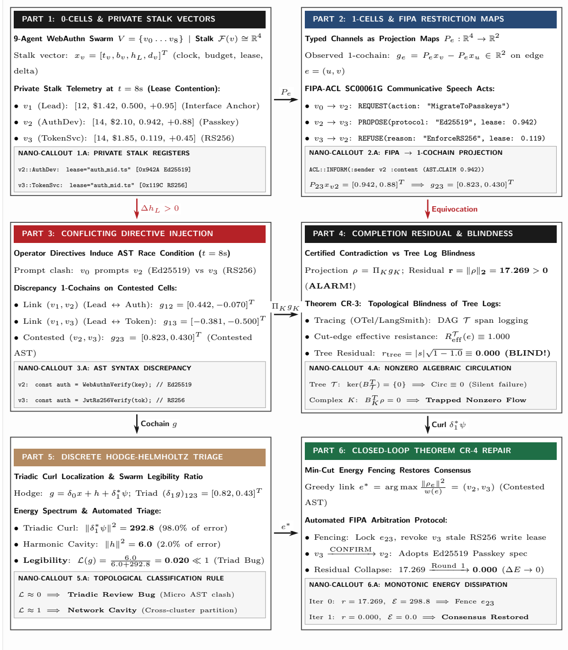
Figure 6: The Complete Closed-Loop Cohomological Control Cycle on a 9-Agent Production Swarm. The 6-part narrative tracks the WebAuthn passkey refactor through private stalk emission (Part 1), FIPA communicative cochains (Part 2), operator fault injection (Part 3), topological residual detection vs. acyclic logging blindness (Part 4), simplicial Hodge-Helmholtz triadic curl localization (Part 5), and Theorem CR-4 greedy closed-loop repair (Part 6).
