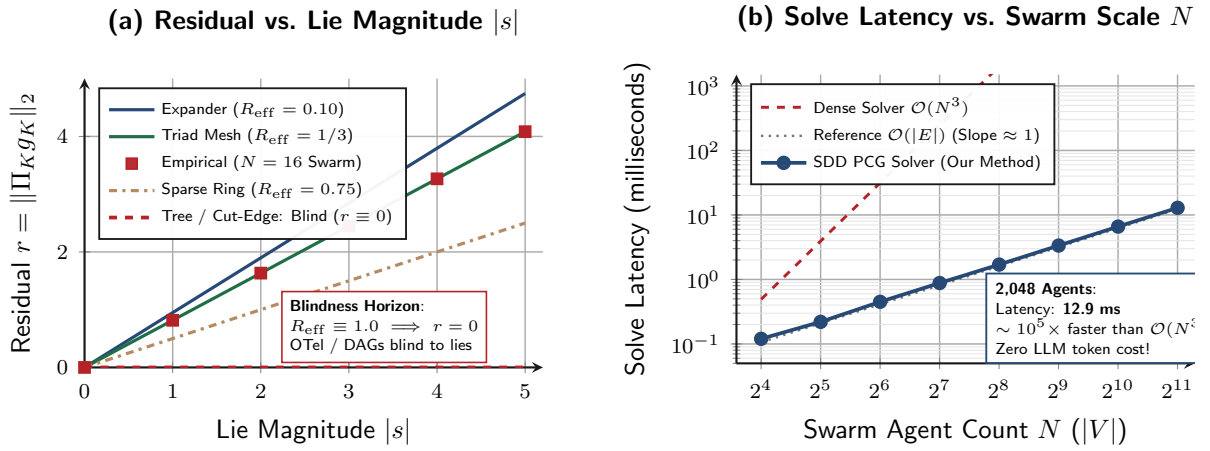
Figure 7: Numerical verification of Theorems CR-1 through CR-3 and computational scalability. (a) Residual r against lie magnitude |s| across topological families: dense expander ( R_{\text{eff}} = 0.10 ), triadic review mesh ( R_{\text{eff}} = 1/3 ), sparse ring ( R_{\text{eff}} = 0.75 ), and cut-edge tree bridge ( R_{\text{eff}} = 1.00 ). While simplicial complexes scale with sensitivity \sqrt{1 - R_{\text{eff}}(e)} , tree-structured logging DAGs are completely blind ( r \equiv 0 ). (b) Empirical solve latency of SDD Laplacian preconditioned conjugate gradient (PCG) solver from N = 16 to N = 2,048 agents ( \sim 12.9 ms at 2,048 nodes), demonstrating near-linear \tilde{\mathcal{O}}(|E|) scaling compared to cubic \mathcal{O}(N^3) state estimation.
