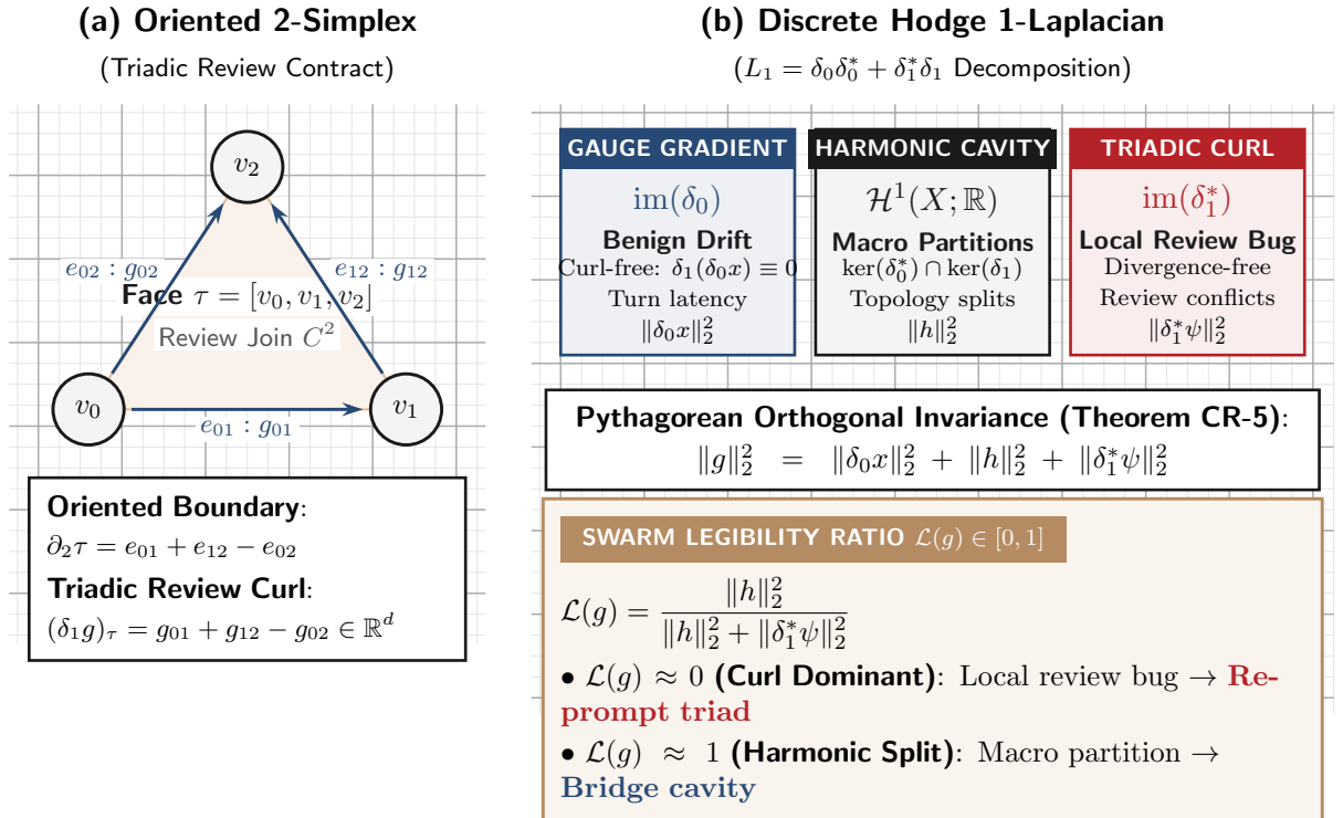
Figure 4: Discrete Hodge decomposition on a simplicial 2-complex. (a) A 2-simplex \tau = [v_0, v_1, v_2] modeling a 3-way review contract with oriented boundary \partial_2 \tau = e_{01} + e_{12} - e_{02} . (b) The Hodge 1-Laplacian L_1 = \delta_0 \delta_0^* + \delta_1^* \delta_1 decomposes observed discrepancies into mutually orthogonal gauge gradients ( \text{im}(\delta_0) , blue), harmonic cavities ( \mathcal{H}^1 , dark), and triadic curls ( \text{im}(\delta_1^*) , red), yielding the zero-token Swarm Legibility Ratio \mathcal{L}(g) .
