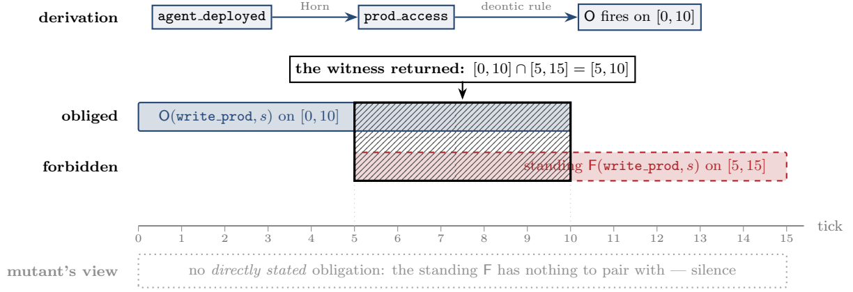
Figure 3: The witness, drawn — the canonical instance the propagation-free mutant misses. Unit propagation forces prod_access from the deployed fact, which fires O(\text{write\_prod}, s, [0, 10]) ; the standing prohibition covers [5, 15] ; and the keyed sweep-line hands back the hatched overlap [5, 10] together with the two fired rules — an object a human can argue with, not a verdict. The dotted lane is the same policy set as seen by a checker that never propagates: the obligation is never derived, so there is no pair to clash and the scanner stays silent. This is the species of conflict whose absence flips the verdict on 100 of the 885 conflicting policy sets in the sweep [internal, b4_deontic_fragment.py , seed 20260816].
