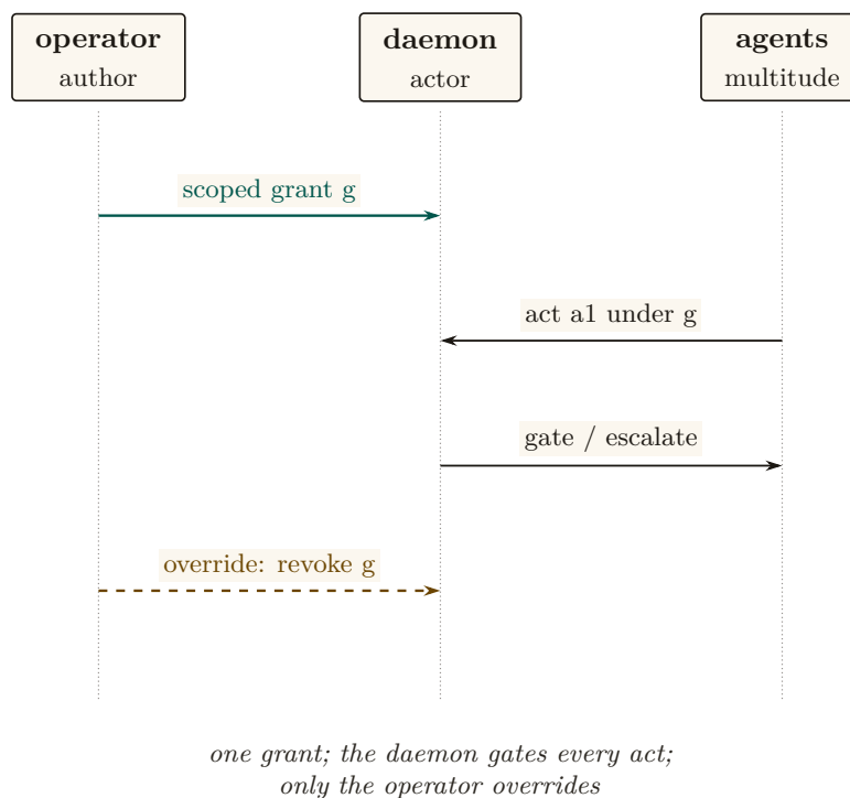
Figure 7: The grant-and-gate sequence, three lifelines and four messages, no crossing. The operator grants once (message 1: scoped grant g). Agents act under that grant (message 2), and the daemon gates or escalates every such act (message 3) rather than granting again. The override (message 4) is the one edge running straight from operator to daemon, bypassing the agents entirely. Idealized to one representative act; a live fleet repeats messages 2–3 per act, not per grant [internal].
