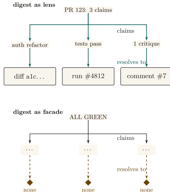
Figure 2: Two claim trees of identical shape. Top: the legible digest’s three named claims each resolve to one artifact — a diff, a test run, a review comment. Bottom: a same-shaped summary whose three claims resolve to nothing an operator can open. A safe summary is an index into evidence; a calm one that terminates early is a Potemkin digest, whichever claim count it advertises [internal].
