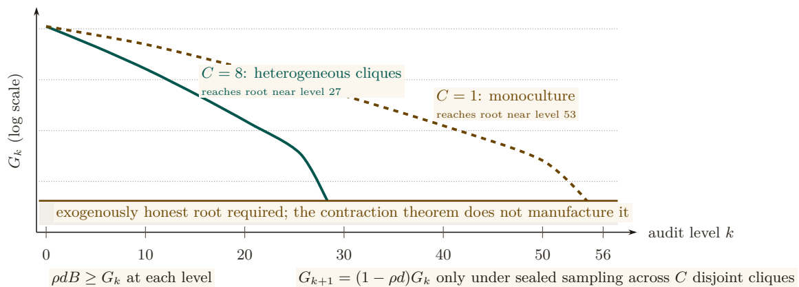
Figure 8: Recursive auditing becomes finite only when corrupt opportunity contracts. The parameterized example plots the chapter’s reported depths: heterogeneous sealed sampling across C = 8 cliques reaches the honest-root boundary near level 27, while a monoculture ( C = 1 ) requires roughly 53 levels. More boxes or more height would not prove this result; the governing conditions are local deterrence \rho dB \geq G_k and contraction G_{k+1} = (1 - \rho d)G_k . The amber floor is deliberately separate: the imported theorem bounds the tower but does not supply its exogenously honest root or the telemetry that estimates d .
