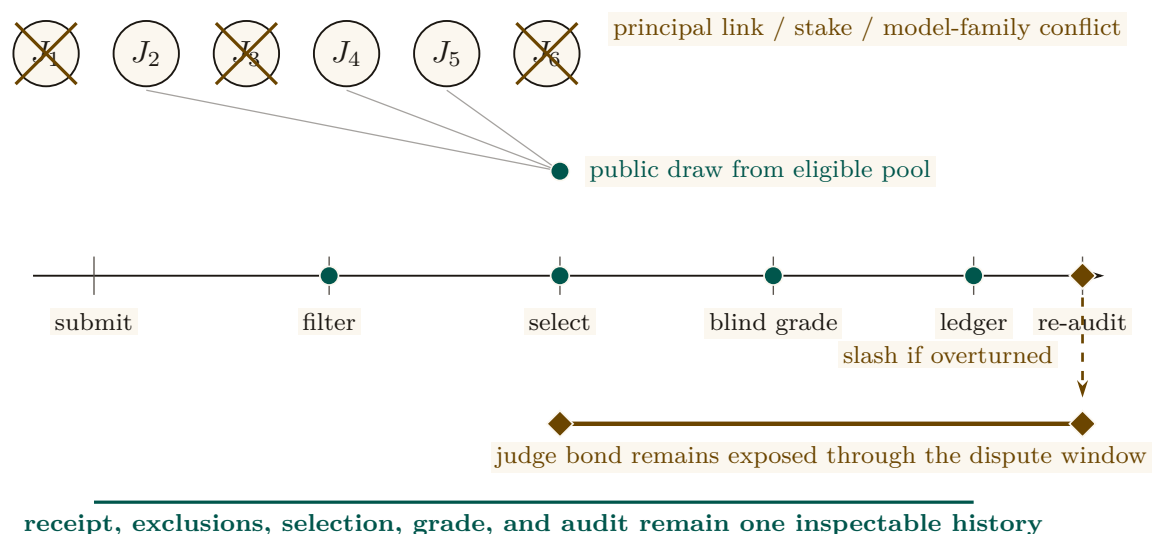
Figure 5.11: The judge market has two different proof moments. Neutrality is earned before selection: candidates sharing a principal, stake, or model family with the graded party are visibly removed, then a public draw selects from what remains. Accountability persists after selection: the judge posts a bond, grades blind, and remains exposed until a later re-audit. The ledger records the receipt, exclusions, draw, grade, bond, and audit, so “neutral” is a checkable history rather than a title attached to the chosen judge.
