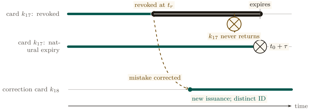
Figure 2.7: Acceptance is a one-way interval attached to one card ID. Card k_{17} stops being admissible either at explicit revocation or at natural expiry and never re-enters the valid set. If revocation was a mistake, the operator issues k_{18} on a new lane; correction creates new authority rather than mutating rejected history.
