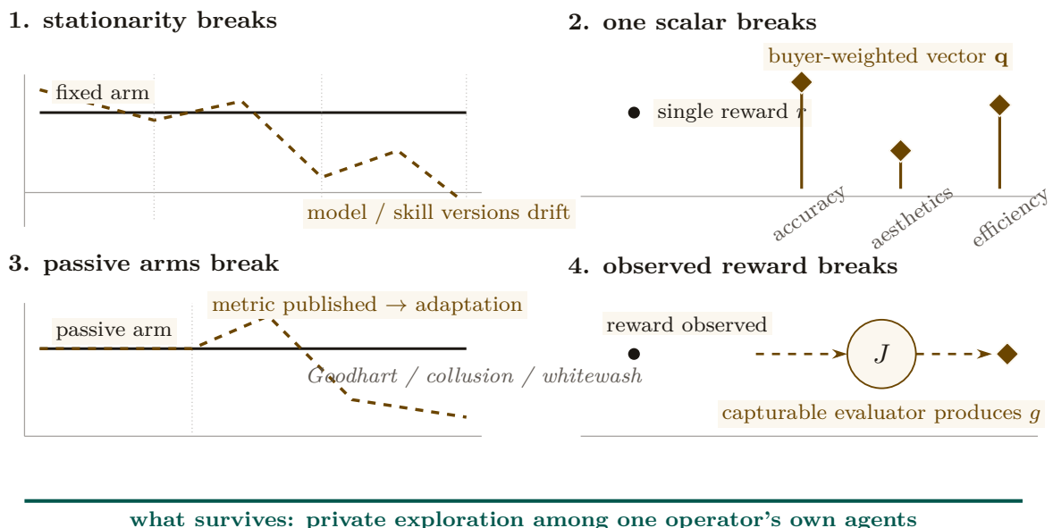
Figure 5.9: Why public reputation is not a bandit problem. Four diagnostic microplots expose the broken assumptions: agent quality drifts across versions; quality is a buyer-weighted vector; strategic actors respond to measurement; and the grade is produced by a capturable evaluator rather than simply observed. Bandit exploration still fits one bounded task—the teal rail, private routing within one operator’s fleet. Exporting the frame to a public market silently assumes away the substrate and mechanism-design problems.
