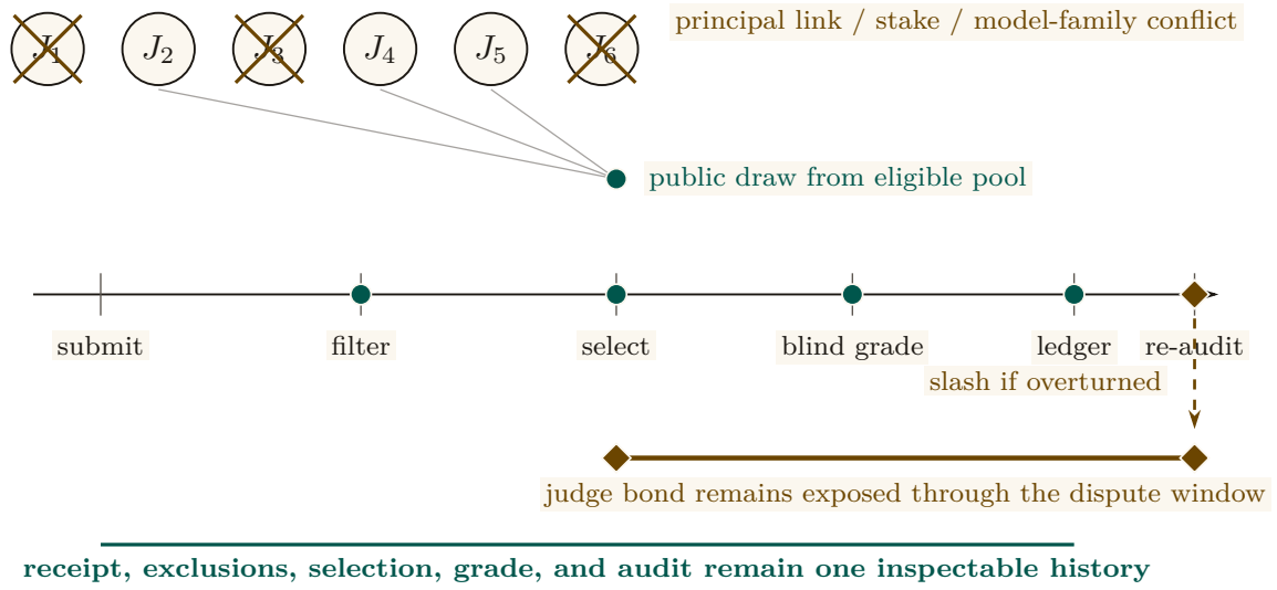
Figure 4.11: The judge market has two different proof moments. Neutrality is earned before selection: candidates sharing a principal, stake, or model family with the graded party are visibly removed, then a public draw selects from what remains. Accountability persists after selection: the judge posts a bond, grades blind, and remains exposed until a later re-audit. The ledger records the receipt, exclusions, draw, grade, bond, and audit, so “neutral” is a checkable history rather than a title attached to the chosen judge.
