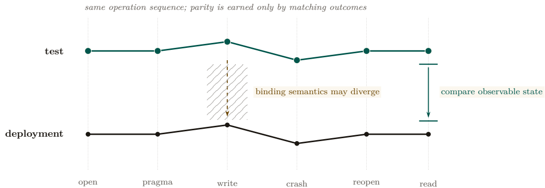
Figure 1.12: Runtime parity as a trajectory comparison. The same operation sequence is applied to the test binding and to the compiled deployment daemon; the harness must compare observable state after reopen, not merely confirm that both programs build. The hatched gap is the unproved surface where pragma, locking, or checkpoint semantics can diverge. A shim aligns interfaces, but only booting the deployment runtime and differential testing can collapse that gap into a verified invariant.
