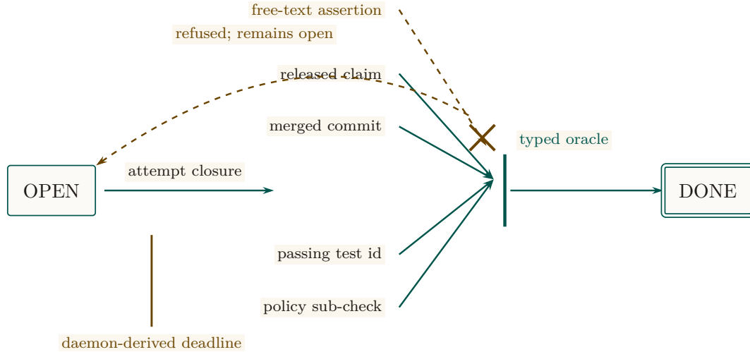
Figure 1.9: Typed evidence passes through a narrow closure aperture. A commitment may close as done only when the daemon can re-check a reference from the finite oracle vocabulary: a released claim, merged commit, passing test identifier, or satisfied policy sub-check. A free-text assertion is deflected back to the open state rather than translated into evidence. The complementary deadline is also daemon-derived; the agent selects the work, not the terms under which its promise becomes easy.
