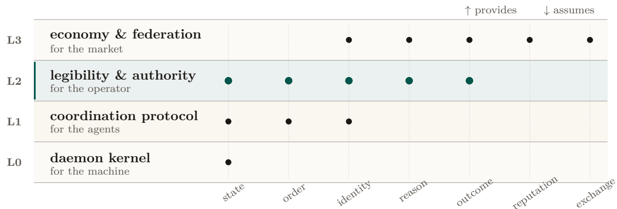
Figure 3.1: The system as four strata rather than four products. Dots mark the capabilities each layer contributes or consumes; alignment exposes reuse across layers. This chapter owns the L2 operator surface and uses the L1 directory substrate. It assumes ordered kernel state below and supplies accountable identity, reasons, and outcomes to reputation and exchange above.
