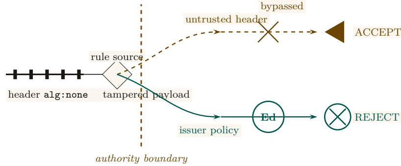
Figure 2.3: Algorithm confusion occurs at the rule-selection boundary, not in the token’s shape. Identical tampered bytes are accepted when the token selects its own verifier and rejected when authenticated issuer policy pins Ed25519. The fork isolates the only causal difference: control of the verification rule.
