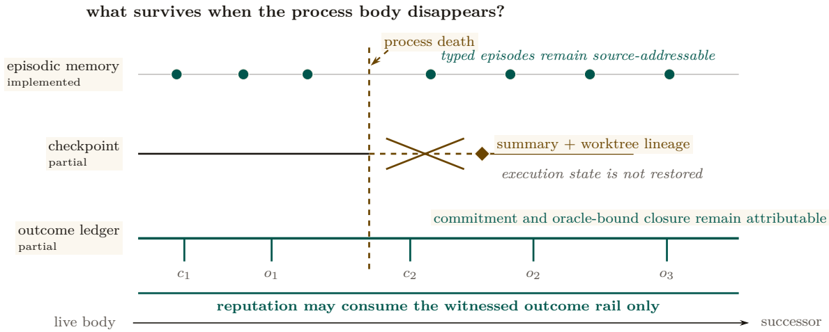
Figure 4.4: The three continuity organs have different survival depths. Episodic memory ( implemented ) retains source-addressable episodes across the death boundary. The checkpoint organ (PARTIAL) preserves a summary and worktree lineage, but the crossed gap marks the execution state it cannot restore. The outcome ledger (PARTIAL) preserves commitments and oracle-bound closures on an unbroken attributable rail. Reputation keys on that lowest rail, not on a recalled episode or a restart summary.
