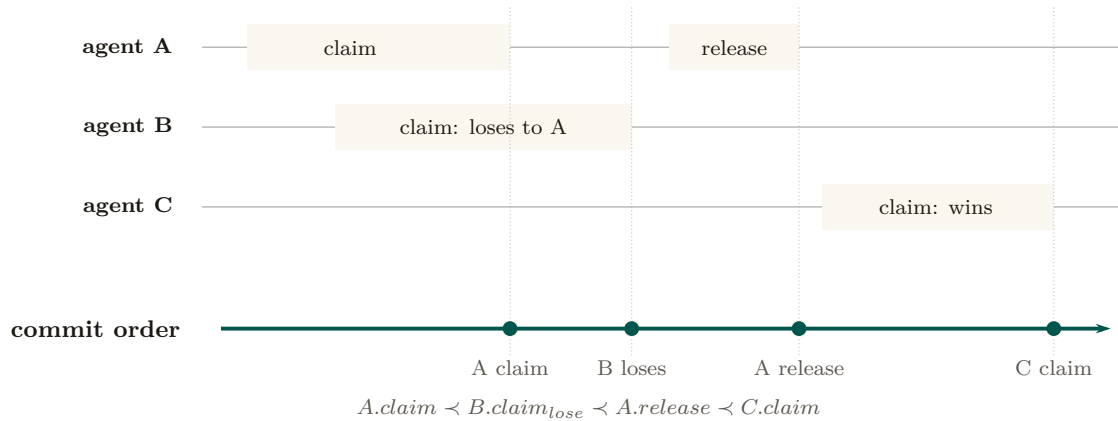
Figure 1.11: A real-time history and its extracted linearization. Operations may overlap in caller time, but each receives one commit point on the single writer’s rail. Those points explain the observable result without a prose table: A wins, B overlaps but loses to the recorded holder, A releases, and only then can C win. The claim is conditional on one writer, no uncommitted reads, and replies after commit; a bypass would destroy the correspondence.
