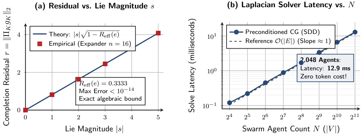
Figure 4: Numerical verification of Theorems CR-1 through CR-3 on synthetic expander meshes conforming to Swiss Modern Systems Graphics. (a) Observed residual r against lie magnitude s on a 16-agent mesh ( R_{\text{eff}} = 1/3 ), confirming the closed form r = |s| \sqrt{1 - R_{\text{eff}}(e)} with relative error < 10^{-14} . (b) Empirical solve latency of SDD Laplacian preconditioned CG solver from N = 16 to N = 2,048 agents, confirming near-linear scaling ( \sim 12.9 ms at 2,048 nodes).
