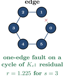
Figure 2: Regime diagram for the mechanism, in one legend with Figure 1 (harborblue solid compared, seagreen dashed relayed, gray dotted severed; the shipred \times marks the lied-on link, independently of its tier). (a) A single-edge fault on a relayed link in a visible cycle gives r = 1.225 for s = 3 . (b) The same fault on a relayed bridge gives r = 0 . (c) A severed edge has no row in K_c and cannot affect this residual. The relayed endpoint claims in (a) and (b) also permit direct sender-claim comparison when authenticated and snapshot-aligned. The figure states a one-edge residual criterion, not a unique detection advantage or a criterion for every split view [internal, sheaf_harness_v2.py].
