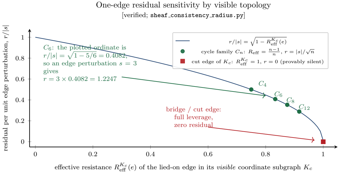
Figure 3: One-edge residual sensitivity is set by the visible topology and chosen Euclidean feature metric. The closed form plots residual per unit edge perturbation , r/|s| = \sqrt{1 - R_{\text{eff}}^{K_c}(e)} , against the effective resistance of the lied-on edge in its visible coordinate subgraph K_c — compared-plus-relayed links only, so severing a link on the edge’s cycle moves the point right, toward silence. The cycle family C_n sits at R_{\text{eff}}^{K_c} = \frac{n-1}{n} ; the marked C_6 point is the plotted ordinate 0.4082, which an absolute lie of s = 3 scales to the harness’s r = 1.2247 . The cut-edge corner R_{\text{eff}}^{K_c} = 1 is provable silence [verified; closed form exact on C_4 – C_{12} and 200 random graphs, sheaf_consistency_radius.py ].
