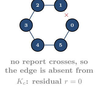
(c) C_6 , lie on a severed edge
