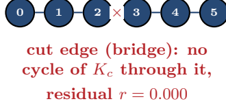
(b) P_6 , lie on a relayed bridge
