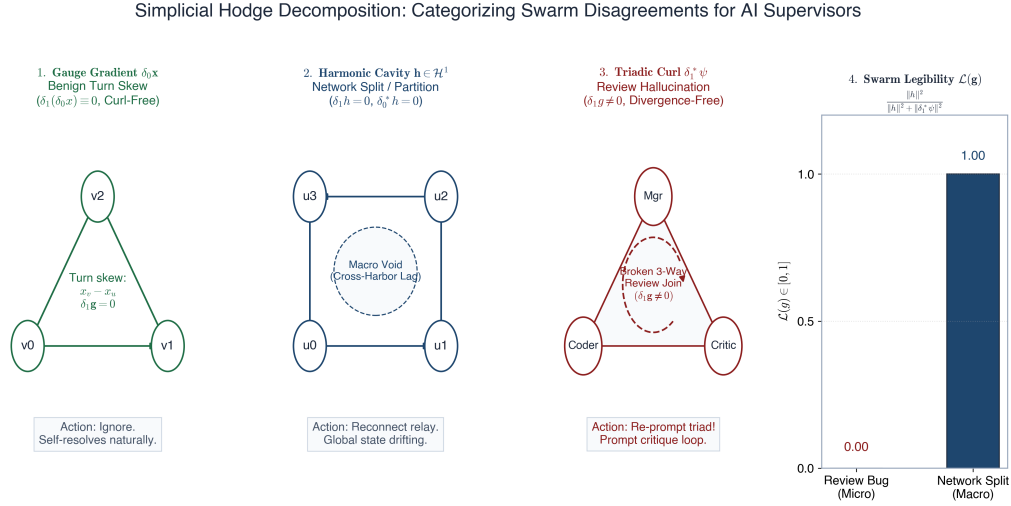
Figure 4: Discrete Hodge-Helmholtz Decomposition on a simplicial 2-complex. An observed cochain g splits into three mutually orthogonal components: gauge gradient \delta_0 x (benign turn lag), harmonic cavity h (macro-partition hole), and triadic curl \delta_1^* \psi (micro-review hallucination). The Swarm Legibility Ratio \mathcal{L}(g) quantifies whether the failure is micro or macro.
