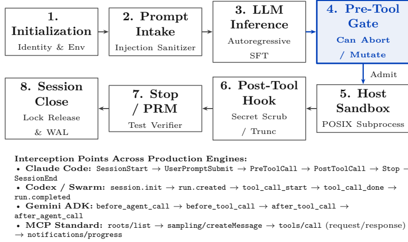
Figure 7: The Agent Lifecycle Hook pipeline and comparative interception points across Claude Code, OpenAI Codex, Google Gemini ADK, and Model Context Protocol (MCP). The Pre-Tool Interception Gate acts as a Ramadge–Wonham supervisory controller ( S/G ), providing the critical effect-boundary enforcement point capable of halting or rewriting unsafe tool calls before OS execution.
