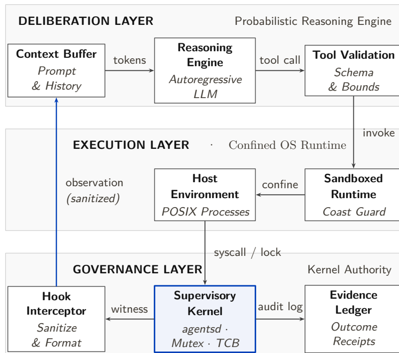
Figure 9: The closed agentic architecture loop: three-layer Swiss stratification separating probabilistic deliberation from deterministic kernel coordination.
