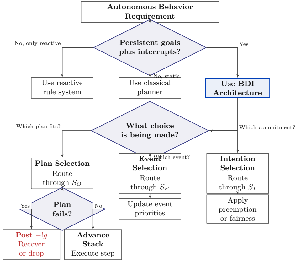
Figure 1: BDI execution flow and operational choice architecture. Adapted from AgentSpeak(L) semantics [?], distinguishing reactive rules, static STRIPS-style planners, and dynamic BDI agents. The three core selection functions ( S_E for events, S_O for applicable plans, and S_I for intention stacks) govern runtime scheduling, with explicit plan failure handling via the -!g recovery event.
