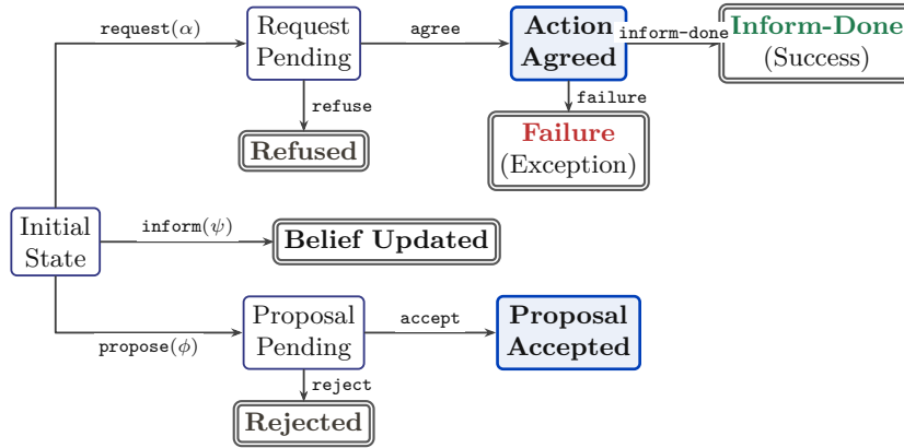
Figure 3: FIPA-00037 Communicative Speech Act state transition machine. Messages are typed performatives governing mental-state preconditions and rational effects across sender and receiver agents.
