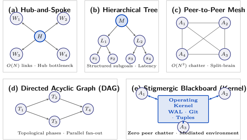
Figure 8: Taxonomy of Multi-Agent Swarm Topologies. While peer-to-peer swarms suffer from O(N^2) message inflation and consensus failure, the Stigmergic Blackboard coordinates agents via environmental state mutations mediated by the authoritative operating kernel.
