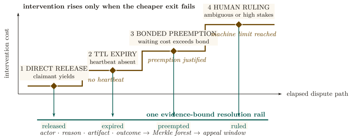
Figure 2: Dispute resolution is an escalation staircase. The system first offers a zero-coercion exit, then waits for the claimant’s TTL, then permits priced preemption, and reaches human judgment only after the machine-readable options are exhausted. Every station can terminate the dispute, and every termination descends to the same evidence rail. Escalation therefore changes the decision cost and decision-maker without discarding the record needed for appeal.
