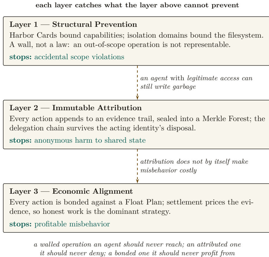
Figure 1: The commons authority’s three layers of trust, read top to bottom as a defense-in-depth stack: each layer catches exactly what the layer above it structurally cannot. Structural prevention (§3) makes an out-of-scope operation unrepresentable, but an agent with legitimate access can still write garbage; immutable attribution (§4) makes every action traceable to a bonded principal even after the acting identity is discarded, but a traceable action is not thereby a costly one; economic alignment (§7) closes that gap by pricing the evidence the first two layers produce. No single layer is complete on its own — the guarantee is the composition. [internal]
