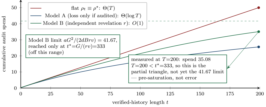
Figure 3: Cumulative audit spend against verified-history length t under the three incentive-compatible schedules of Theorem 3, at the running parameters. Flat auditing (shipred) grows linearly; Model A (harborblue) grows logarithmically; Model B (seagreen) approaches the closed-form limit aG^2/(2dBrv) = 41.67 but has not reached it by the measured horizon T=200 , since saturation requires t^* = G/(rv) = 333 — the gap between the measured 35.08 and the limit is pre-asymptotic, not error [internal, b2-tower.py].
