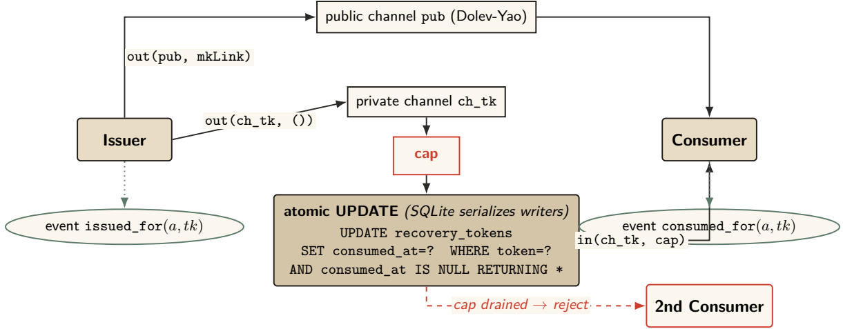
Figure 8: Magic-link single-use atomicity. The SQL UPDATE ...WHERE consumed_at IS NULL RETURNING is the runtime analogue of the ProVerif private-channel cap: SQLite serializes concurrent writers, so the first caller drains the cap and the second consumer’s transaction returns zero rows. Verified properties: injective single-use ( \text{inj-event}(\text{consumed\_for}) \Rightarrow \text{inj-event}(\text{issued\_for}) ) and binding.
