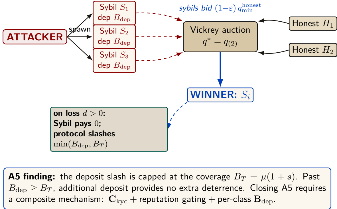
Figure 5: Sybil attack flow. The attacker spawns K Sybil identities, each posting deposit B_{\text{dep}} , then undercuts honest bids by \varepsilon and defaults on loss. The protocol confiscates the Sybil’s deposit on default, but the slash amount is capped at the coverage B_T — so beyond B_{\text{dep}} \geq B_T additional deposit provides no extra deterrence. Empirically demonstrated in Figure 6.
