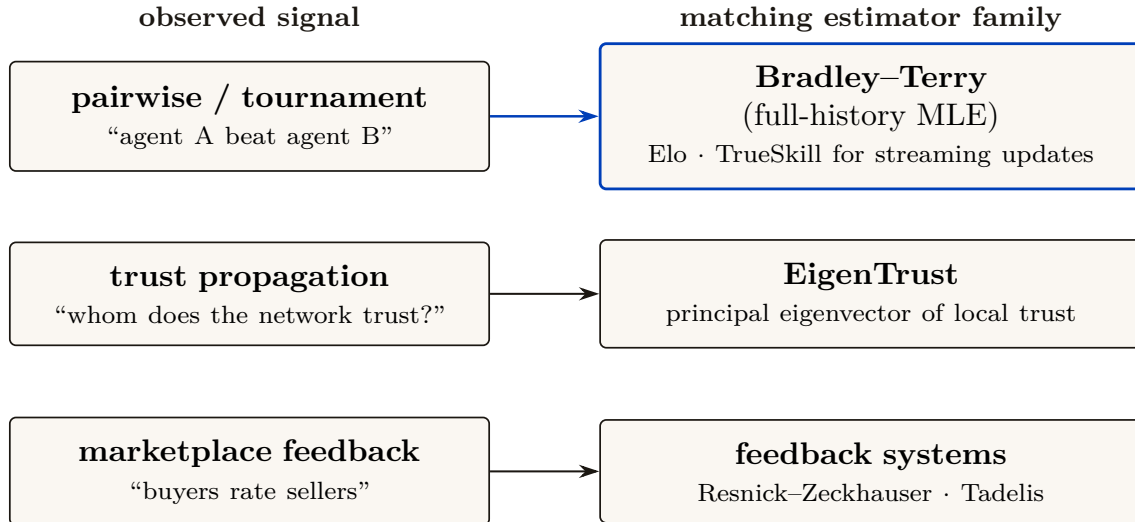
Figure III.8: The estimator family, by signal type — the wrong choice is a real error. Pairwise outcomes call for Bradley–Terry / Elo / TrueSkill; network trust calls for EigenTrust (PageRank for reputation — not a bandit); marketplace feedback calls for feedback systems with measured price premia (Resnick–Zeckhauser’s ~8%; Tadelis on adverse selection). A SQLite harbor holds the whole settled-outcome history, so it is in the Bradley–Terry regime, not the streaming-Elo regime. None of these is the hard part: the estimator is cheap and last , while the substrate beneath — non-forgable identity, continuity, an oracle-witnessed ledger — is the gate.
